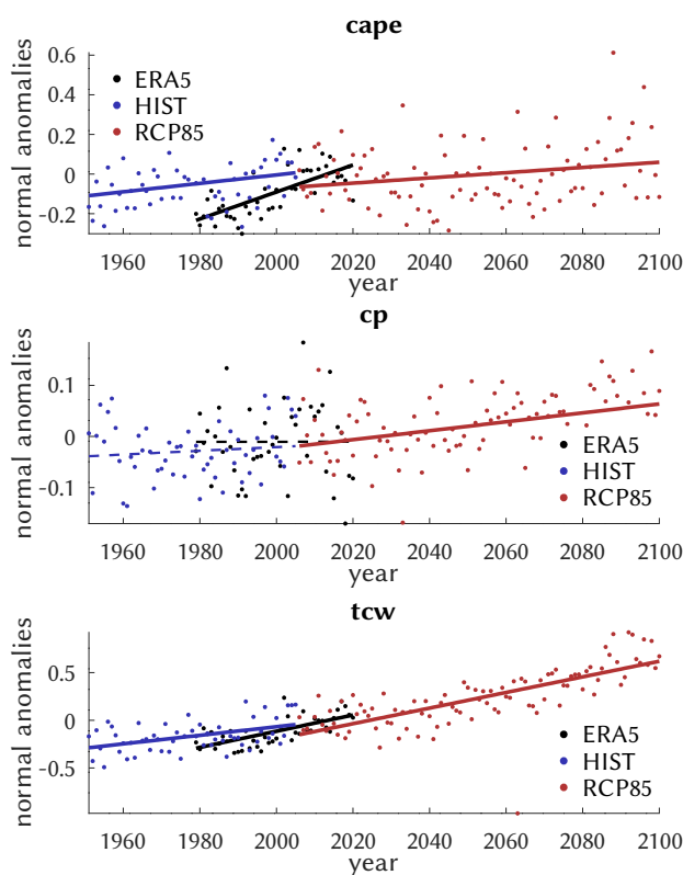
Figure 9. Similar to Fig. 8, for the predictor series and including ERA5 (black) as they enter the classification (normalized). The trends pertain to the full available series, and significance is indicated by solid vs. dashed lines.
