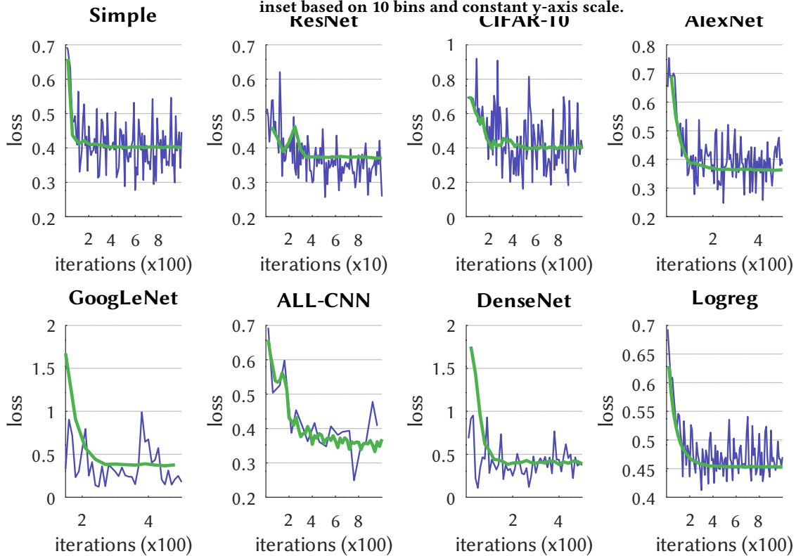
Figure 4. As Figure 2, for the other DL networks (using blue for Train and green for Test).
