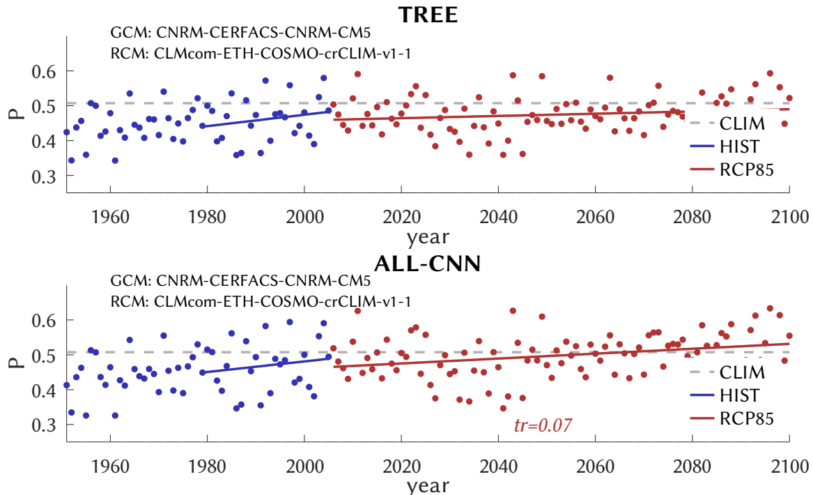
Figure 8. Similar to Figure 7, as simulated by GCM/RCM, for historic (blue) and future (red) emissions. For reference, the observed 2001–2020 climatology is also shown (CLIM, gray dashed).
