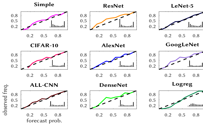
Figure 10. Like Fig. 3, for the deep methods.
