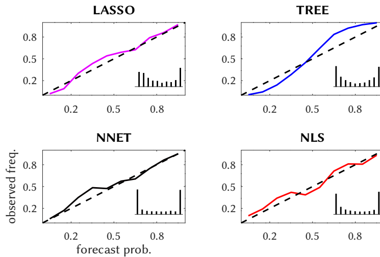
Figure 3. Reliability diagram for the shallow methods, with forecast histogram inset based on 10 bins and constant y-axis scale.
