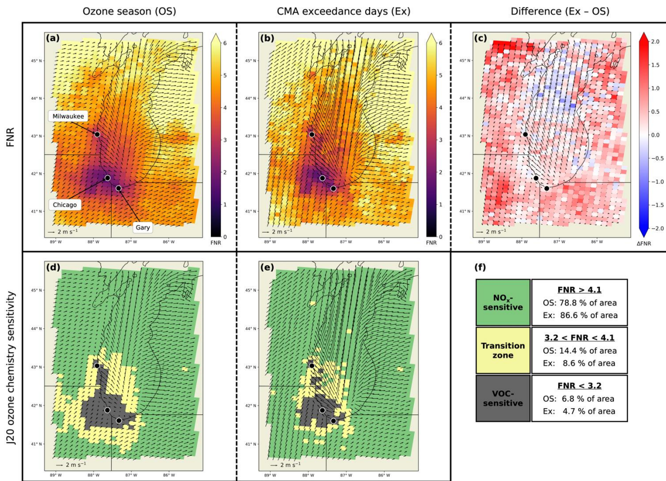
Figure 6. TROPOMI-derived 2019–2021 FNR values in the Lake Michigan region during: (a) the ozone season (OS), (b) Chicago ozone exceedance days (Ex), and (c) the difference between them (Ex – OS). J20 threshold interpretation of 2019–2021 ozone chemistry sensitivity during: (d) the ozone season, (e) Chicago ozone exceedance days, and (f) the percent of the domain area classified as each J20 sensitivity regime. Mean 10-meter winds are represented by arrows.
