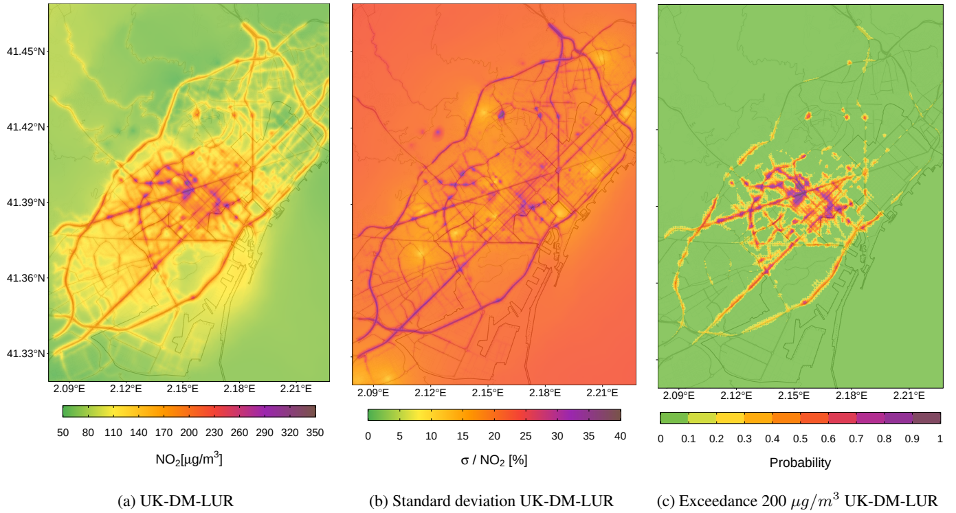
Figure 11. (a) Hourly NO 2 concentration map resulting of applying the UK-DM-LUR methodology at 9h UTC on 28/02/2019. (b) Relative uncertainty associated with the predictions in (a). (c) Hourly probability map of exceeding the 200 \mu\text{g}/\text{m}^3 NO 2 hourly averaged limit using the values in (a) and (b).
