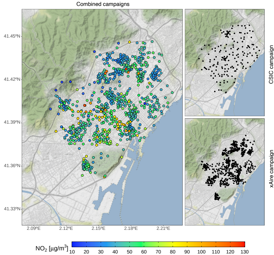
Figure 3. Sampler locations of the two different \text{NO}_2 experimental campaigns used to train the microscale-LUR model. The left panel shows the \text{NO}_2 values and the locations of the combined campaigns. The top- and bottom-right panels show the CSIC and xAire campaign locations, respectively. The colour scale refers to the 2017 annualized \text{NO}_2 values, in \mu\text{g}/\text{m}^3 . The map has been generated using ggplot2 (Wickham, 2016) and ggmap (Kahle and Wickham, 2013) R packages (R Core Team, 2013), and data from OpenStreetMap. © OpenStreetMap contributors 2017, distributed under the Open Data Commons Open Database License (ODbL) v1.0. Map tiles by © Stamen Design, under a Creative Commons Attribution (CC BY 3.0) license.
