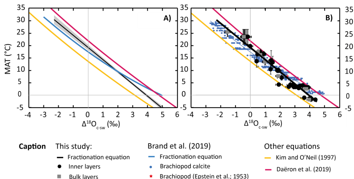
Figure 2: Plot comparison of A) regression lines for different temperature-oxygen isotope fractionation for brachiopod calcite (This study, Brand et al. 2019), laboratory precipitated calcite (Kim and O'Neil, 1997) and slow growing cave calcite (Daëron et al., 2019) and B) corresponding datasets for brachiopod calcite (modified after Brand et al., 2019). Uncertainty envelope 95% CI of the York least square regression (York et al., 2004).
