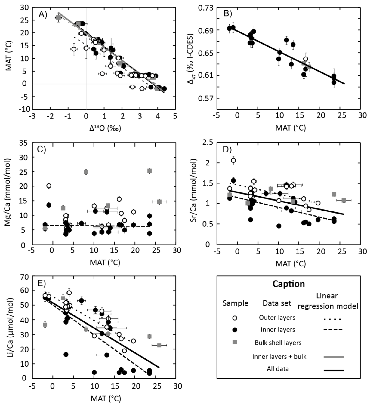
280 Figure 1: Geochemical data and linear regression model for each geochemical parameter tested for its relationship with brachiopod living temperature. Parameters associated with each regression model are listed in table 3.
