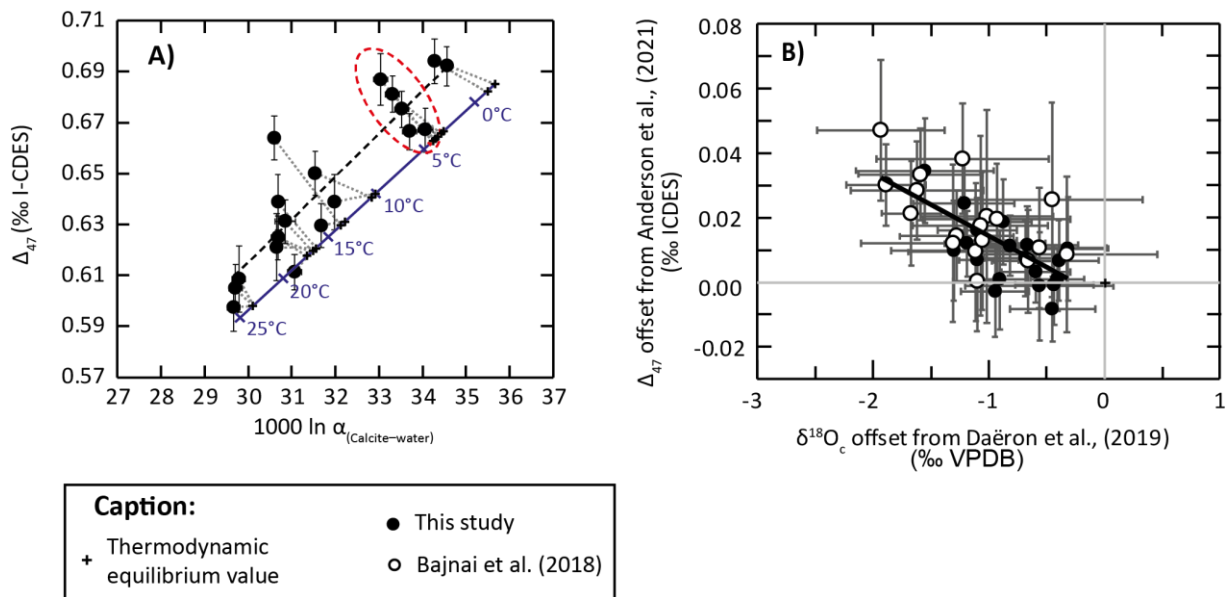
Figure 57: Non equilibrium fractionation and kinetic effects in brachiopod shell calcite as evidenced by clumped isotopes and oxygen isotopes. A) Plot of brachiopod inner shell layers in the \Delta_{47} - 1000 \ln \alpha_{(\text{calcite-water})} space compared with the equilibrium line (blue line) defined by very slow growing abiogenic calcite (Daëron et al., 2019; Anderson et al., 2021). Red highlight, results from A. kerguelensis (Crozet Islands) and their expected geochemical values on the equilibrium line. Note the negative correlation between \Delta_{47} and 1000 \ln \alpha_{(\text{calcite-water})} evidenced in this subset. B) \delta^{18}\text{O}_c and \Delta_{47} offset from their expected equilibrium values calculated from environmental parameters using the equations of Daëron et al. (2019) and Anderson et al. (2021), respectively. The trends in followed by these offsets within our new dataset, is similar to what has been that reported from other brachiopod samples by Bajnai et al. (2018).
