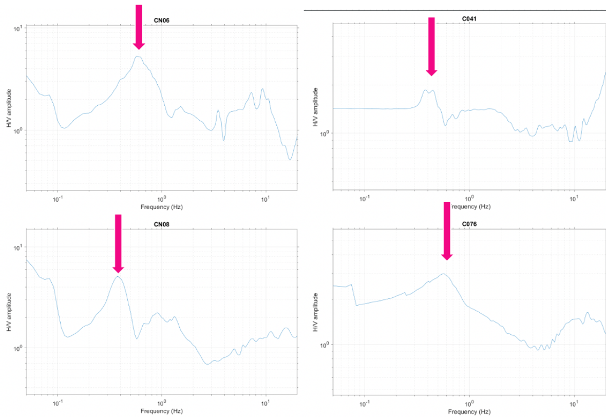
5 Figure S1: Representative H/V measurements at broad-band stations (left panels) and seismic nodes (right panels).
