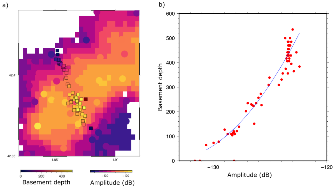
Figure S2: a) Correlation between seismic power amplitudes measured in our dataset and the basement depth estimations from Gabàs et al. 2016. Squares show the basement depth estimations by Gabàs et al 2016, while circles shows the power amplitude in our dataset, measured in dB. Color palettes have been chosen to visualize the correlation between both datasets b) Adjustment between seismic power amplitudes and seismic power amplitudes. Blue line shows the degree 2 polynomial adjustment.
