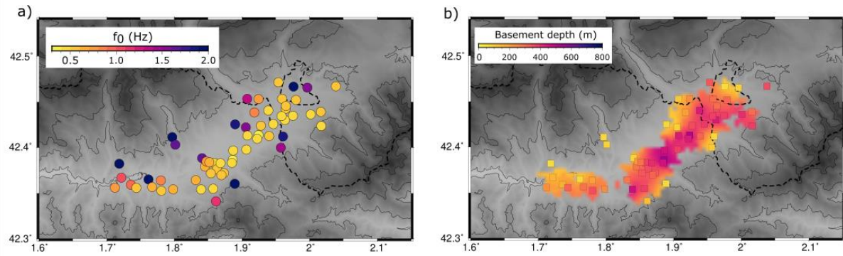
Figure 6: Results from HVSR. a) f_0 values retrieved from broad-band stations and seismic nodes. b) Basement depths estimated from the f_0 values using the scaling law proposed by Gabàs et al. (2016). The background shows the topography and the dashed line corresponds to the Spanish-French border.
