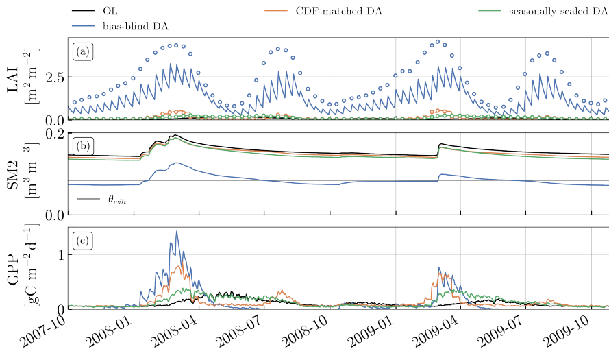
Figure 9. Time series of (a) LAI, (b) SM2 (10-40 cm), and (c) GPP for all DA runs for the Nile delta example grid cell ( 31.125^\circ , 30.875^\circ ). Panel (a) includes the (potentially rescaled) observations that were assimilated in each run (coloured dots, dot colours correspond to line colours).
