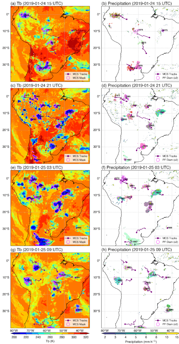
Figure 9. Example MCS tracking from a WRF simulation with 4-km grid spacing showing (a) IR T_b , and (b) precipitation every 6 hours. The magenta contour in (a) and the color shadings behind large clusters of PFs in (b) denote MCS masks. The purple color lines are MCS tracks, the purple dots are MCS initiation locations, and the numbers are MCS track numbers. The magenta circles in (b) show the largest PF equivalent diameter (multiplied by 2 for visibility) within an MCS. An animation with hourly resolution of this event is provided in the supplementary.
