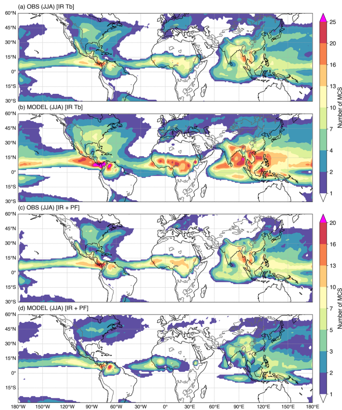
555 Figure 13. Example maps of 20-year mean MCS density during June-July-August for observations and E3SM model outputs as defined by using (a-b) only infrared brightness temperature (IR T_b ) and (c-d) both IR T_b and precipitation feature (PF). Gray contours in the background are topography higher than 1000 m ASL.
