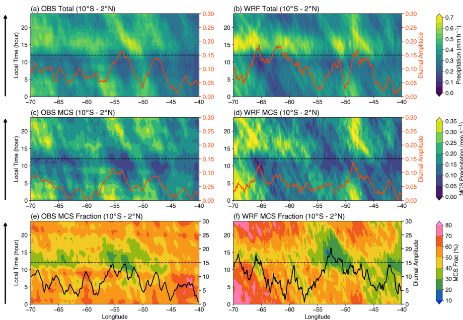
Figure 12. Diurnal cycle of precipitation as a function of longitude during December-March for (a-b) total precipitation, (c-d) MCS precipitation, and (e-f) fraction of MCS precipitation. Precipitation is averaged in the latitude dimension over the central Amazon region (10°S - 2°N, see Figure 11). Orange lines (a-d) and black lines (e-f) show the first harmonic of the diurnal cycle composite amplitude along each longitude.
