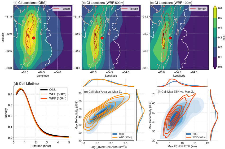
285 Figure 5. Example convective cell tracking statistics. Convection initiation location kernel density estimates (KDE) from (a) radar observations, and WRF simulations with (b) 500-m grid-spacing and (c) 100-m grid-spacing. Color contours in (a-c) are terrain heights (500-m interval starting from 500-m altitude MSL in white), and the red dot is the radar location. (d) KDE of cell lifetime, and joint KDEs of (e) maximum cell area and maximum reflectivity, and (f) maximum 20 dBZ echo-top height and maximum reflectivity. In (e-f), shadings are from observations and contours are from simulations with marginal distributions also shown. The maximum cell area, reflectivity and echo-top heights are obtained over the lifetime of each cell.
