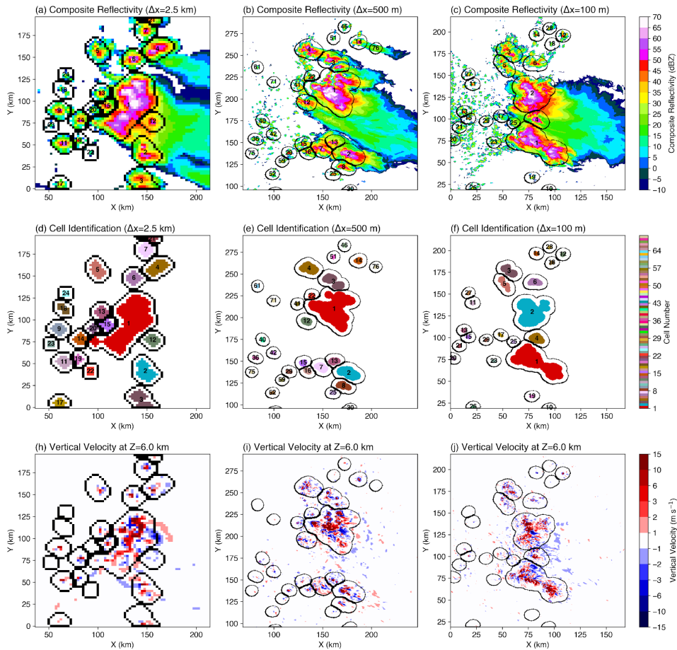
230 Figure 2. Convective cell identification example from WRF simulations at horizontal grid spacings of 2.5 km (left column), 500 m (middle column), and 100 m (right column). The domain size shown is the same across the three simulations (~200 km × 200 km). (a-c) Composite reflectivity, (d-f) convective cell masks, (h-j) vertical velocity at 6-km altitude MSL. Numbers in the cell centers in (a-f) are the labeled cell numbers. Black contours show convective cell mask boundaries expanded outward to a 5-km radius.
