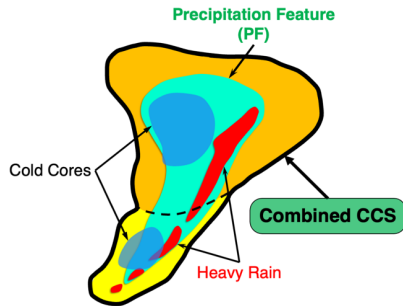
Figure 6. Schematic to identify cold cloud systems (CCS) using T_b and precipitation. (a) Cold cores (contiguous area with T_b < T_{b\text{-threshold-cold}} ) are spread outwards through an iterative dilation process until reaching T_b\text{-threshold-warm} to identify and label CCSs (black contours), (b) CCSs that share a coherent precipitation feature (PF, contiguous area with precipitation rate > threshold) are combined (thick black contour).
