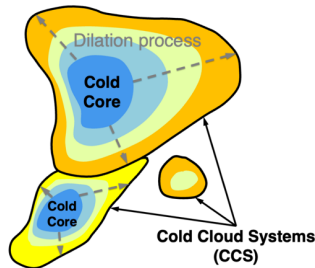
Figure 6. Schematic to identify cold cloud systems (CCS) using T_b and precipitation. (a) Cold cores (contiguous area with T_b < T_{b\text{-threshold-cold}} ) are spread outwards through an iterative dilation process until reaching T_b\text{-threshold-warm} to identify and label CCSs (black contours), (b) CCSs that share a coherent precipitation feature (PF, contiguous area with precipitation rate > threshold) are combined (thick black contour).
