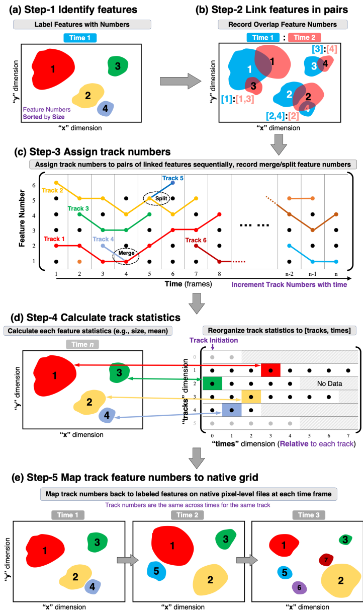
105 Figure 1. PyFLEXTRKR general workflow. (a) Identify and label features on input 2D grid, (b) link features in pairs of adjacent times, (c) assign track numbers, (d) calculate track statistics, (e) map track numbers back to input 2D grid. See Section 2.1 for more details.
