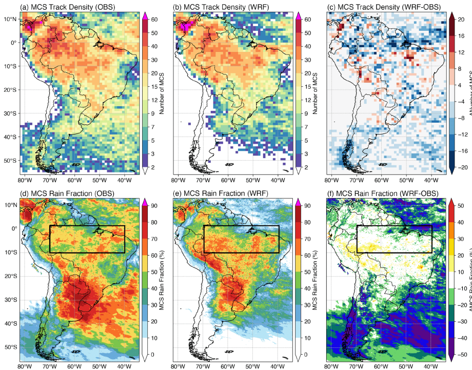
495 Figure 11. Annual MCS track density from (a) observations and (b) WRF with (c) differences (WRF – observations). Annual mean fraction of MCS precipitation to total precipitation from (d) observations and (e) WRF with (f) differences (WRF – observations). The black box in (d-f) shows the region used for the diurnal cycle analysis in Figure 11.
