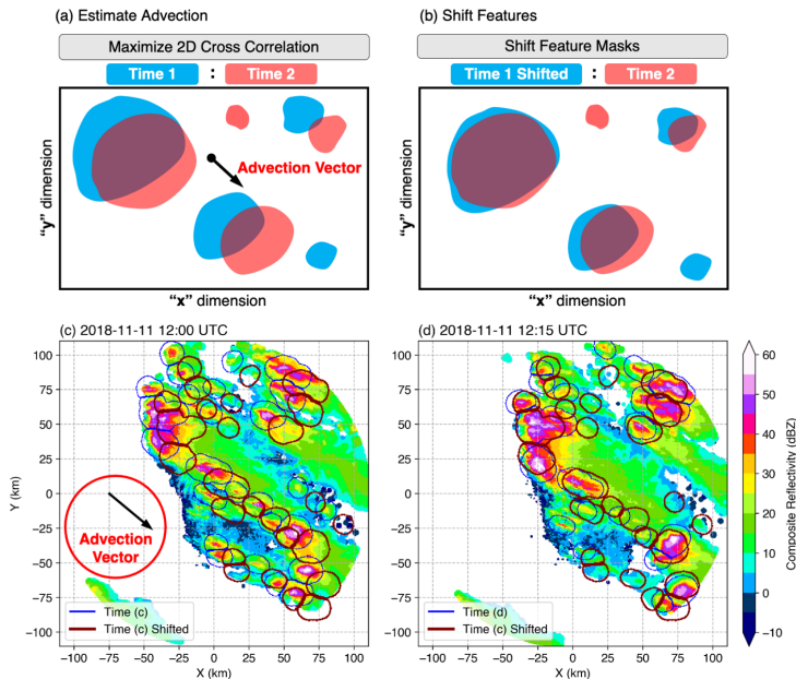
235 Figure 3. Schematic of mean advection estimate by (a) using the 2D cross correlation method between Time 1 and Time 2, and (b) shifting the cell masks from Time 1 and overlaying them on those in Time 2. An example application on actual data is shown in (c-d): shadings are composite reflectivity from two radar scans 15 min apart, contours of convective cells at the two respective times are shown in blue, and the cell masks shifted by the mean advection are shown in dark red.
