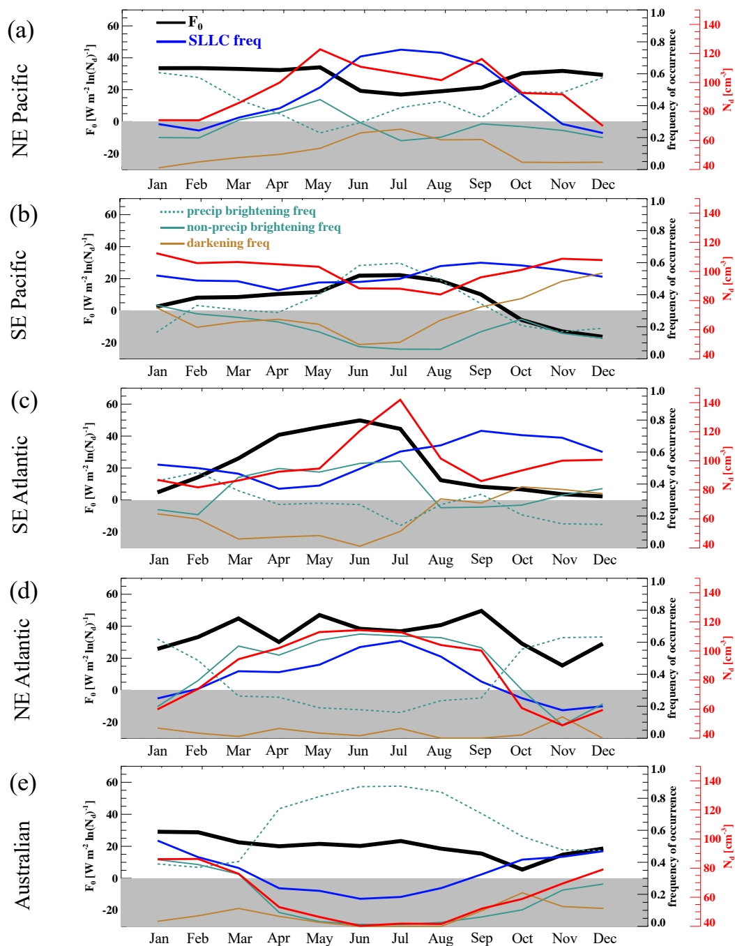
Figure 7. Monthly mean radiative susceptibility ( F_0 ; black), frequency of occurrence of SLIC (blue), monthly mean N_d (red), and the frequency of occurrence of the 3 susceptibility regimes: non-precipitating brightening (solid green), darkening (brown), and precipitating brightening (dotted green). Rows (a–e) represent results for the NE Pacific, SE Pacific, SE Atlantic, NE Atlantic, and the Australian stratocumulus regions, respectively.
