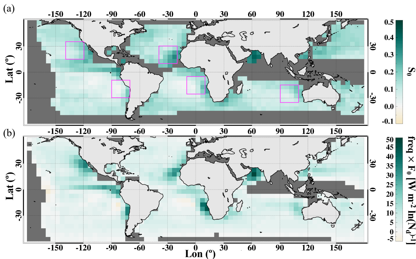
Figure 1. Geographical distribution of marine low-cloud (a) albedo susceptibility ( S_0 ) and (b) the product of radiative susceptibility ( F_0 ) and annual frequency of occurrence of single layer liquid cloud (SLLC). Spatial-temporal averages of 5^\circ \times 5^\circ areas are shown. Only areas with SLLC frequency of occurrence greater than 0.1 are shown in (a). Magenta boxes in (a) indicate five 20^\circ \times 20^\circ marine stratocumulus regions analyzed further in this study
