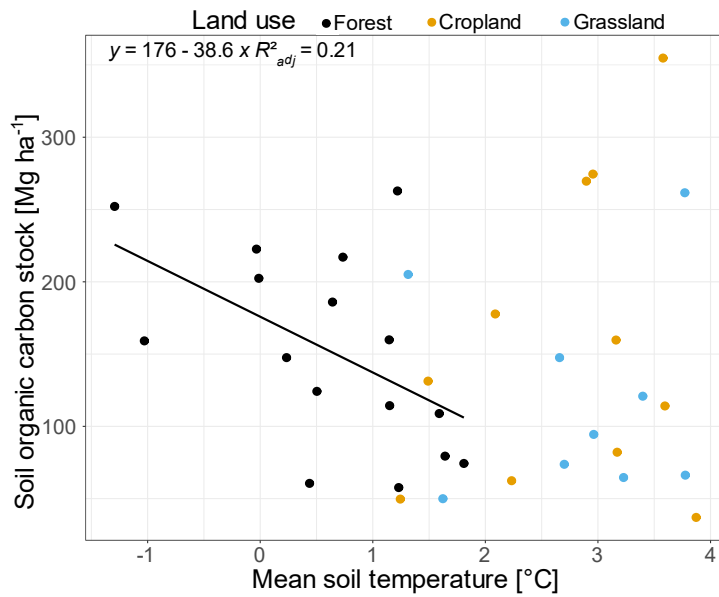
Figure 8: Soil organic carbon (SOC) stocks between 0-80 cm depth [Mg/ha] and mean soil temperature [°C] of forest, grassland and cropland soils with a significant ( p < 0.05 ) correlation (solid line) between SOC stocks and soil temperature in forest soils. Mean temperature was calculated from soil temperatures at 10 and 50 cm.
