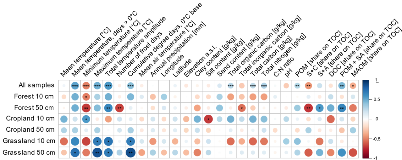
195 Figure 6: Correlogram of the Pearson's correlation coefficient, showing the correlation of mean potential litter decomposition and the most important soil temperature parameters, site characteristics and soil properties. The size and colour of the points represent the direction and the value of the correlation coefficient. Asterisks indicate statistical significance with * p < 0.05 , ** p < 0.01 and *** p < 0.001 .
