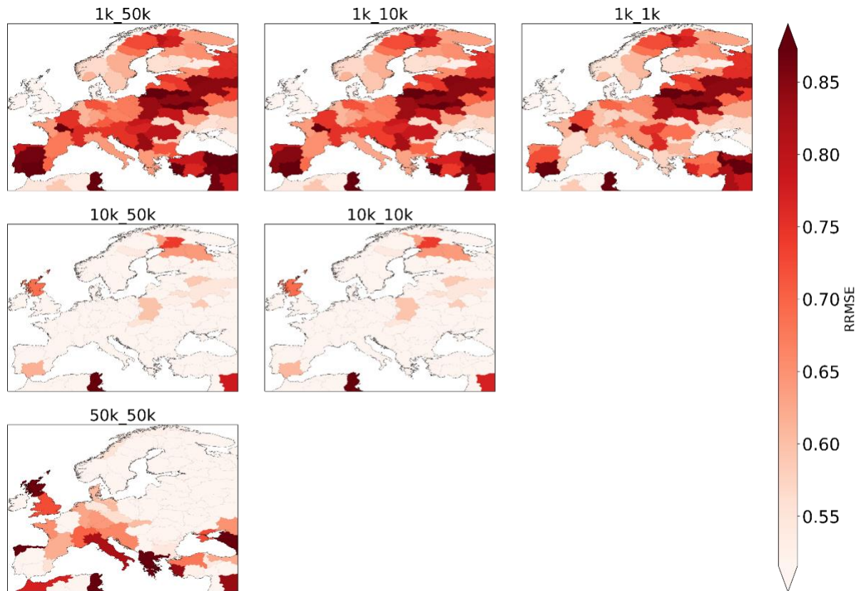
Figure 7: RRMSE values computed per water province based on simulated total evaporation and evaporation data from GLEAM.
