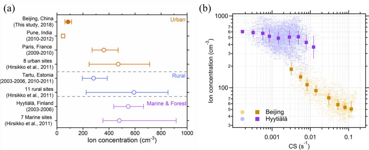
796 Figure 3. (a) Negative cluster ions observed in global urban, rural, forest, and marine sites. The circles represent the 797 median values, and the error bars represent the 25%-75% ranges. Ion mobility ranges for different sites were between sub- 798 1.6 and sub-2 nm. (b) The decreasing trends of the negative cluster ion concentrations with the increase of CS were 799 observed in both Beijing and Hyytiälä. The markers and error bars are median values and 25%-75% ranges, respectively. 800 For comparison, NAIS data were used for both urban Beijing and the clean forest site Hyytiälä. 801
