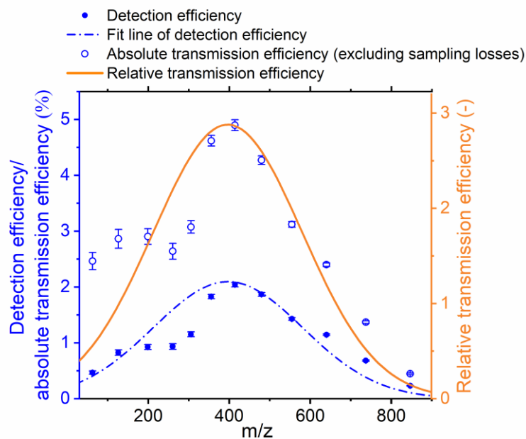
Figure 1. The detection efficiency and absolute transmission efficiency of APi-FTOF determined through the in-situ comparison with NAIS and the relative transmission efficiency of APi-FTOF determined through the depletion method. The relative transmission efficiency is obtained by dividing the detection efficiency by the sampling efficiency of cluster ions. The voltage settings of APi-FTOF remain the same during the experiment.
