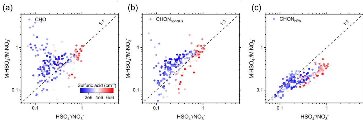
Figure 6. The ratio of \text{CHO} \cdot \text{HSO}_4^- / \text{CHO} \cdot \text{NO}_3^- (a), \text{CHON}_{\text{nonNPs}} \cdot \text{HSO}_4^- / \text{CHON}_{\text{nonNPs}} \cdot \text{NO}_3^- (b), and \text{CHON}_{\text{NPs}} \cdot \text{HSO}_4^- / \text{CHON}_{\text{NPs}} \cdot \text{NO}_3^- (c) as a function of the ratio of \text{HSO}_4^- / \text{NO}_3^- . The color represents the concentration of sulfuric acid.
