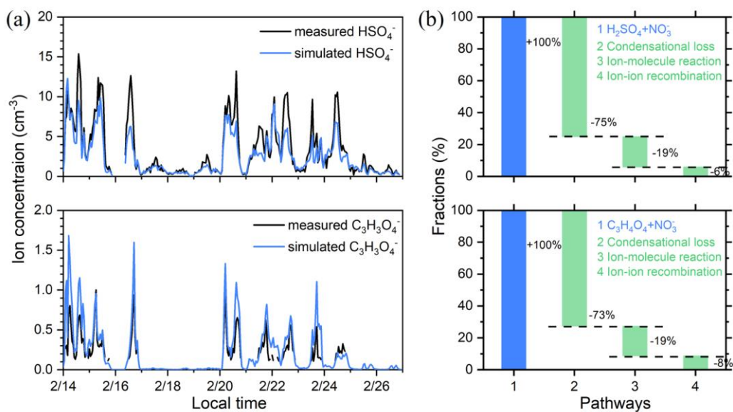
Figure 10. (a) The measured and simulated concentrations of HSO 4 - and C 3 H 3 O 4 - in Beijing. The simulation is performed according to dynamic models as described in Section 2.3 and four formation and loss pathways were considered. (b) The fractions of the formation or loss rates of HSO 4 - and C 3 H 3 O 4 - contributed by different pathways. The average values of the results were shown here.
