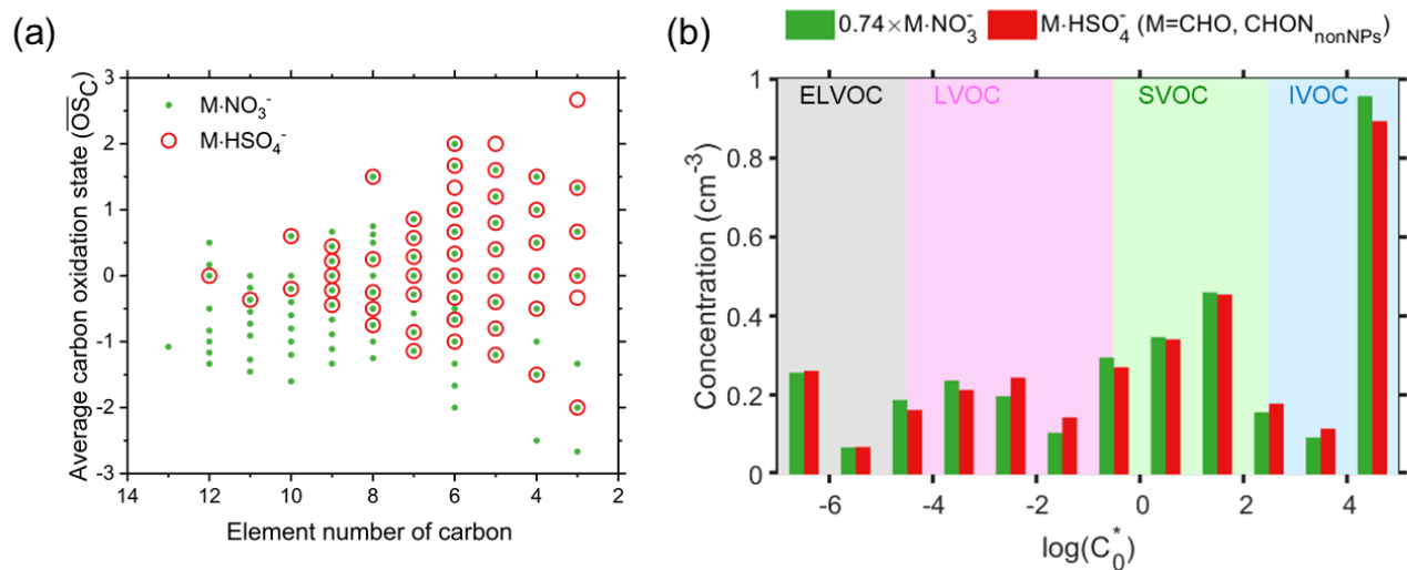
812 Figure 5. (a) The carbon atom number and average carbon oxidation state ( \overline{OS}_C ) of molecules that adduct to NO_3^- and 813 HSO_4^- respectively. (b) The volatility distribution of CHO and CHON_{nonNPs} species in the forms of adducts with both 814 NO_3^- and HSO_4^- . Only species that attached to both NO_3^- and HSO_4^- were considered for calculating the volatility 815 distribution. The volatilities were calculated using the method of Qiao et al. (2021). 816
