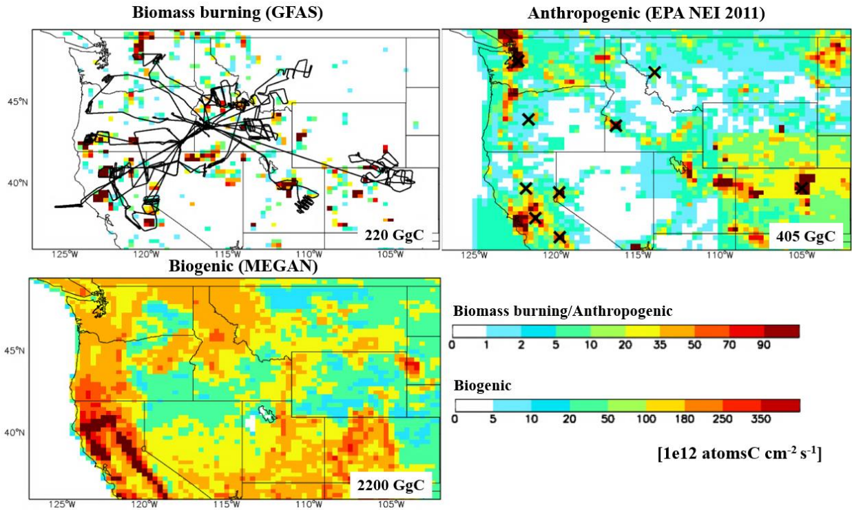
985 Figure 1. VOC primary emissions over the western US in the base GEOS-Chem simulation for the 2018 fire season (JJAS). Also shown are the C-130 flight tracks during WE-CAN (black lines in the top left map), and locations of the ground stations used in this study (black × symbols in the upper right map). Note the color scale for biogenic emissions (MEGANv2.1) is different from that for biomass burning (GFASv1.2) and anthropogenic emissions (US EPA NEI 2011). VOC speciation for biomass burning in the base simulation is provided in Tables 1 and S2.
