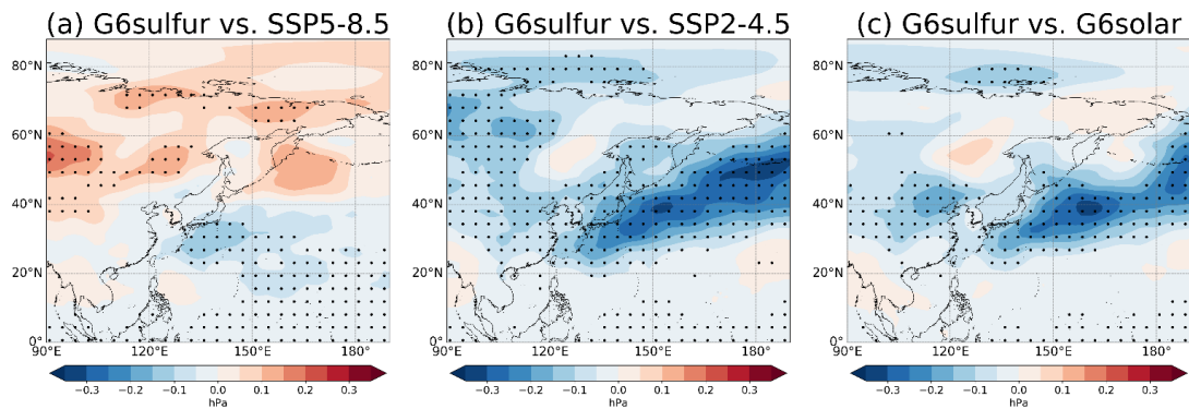
690 Figure 6: As Figure 5 but for distributions of storm tracks (the root-mean-square of 2-6-day bandpass-filtered MSLP, unit: hPa) during MJJAS. Stippling indicates changes that are statistically significant (p-value < 0.05 based on the Student's t-test).
