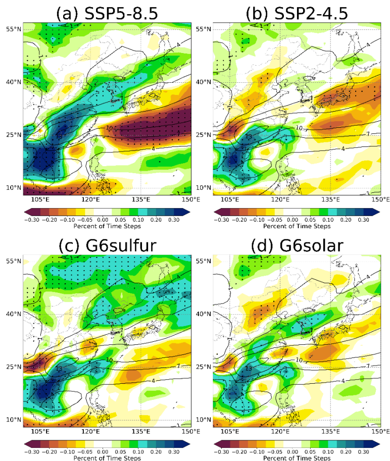
695 Figure 7: Absolute changes (shaded) in annual mean AR frequency (percent of 6-hourly time steps) for the future period of 2071-2100 relative to the historical baseline during 1981-2010. Black contours show the annual mean AR frequency during the historical baseline period. Stippling indicates changes that are statistically significant at a confidence level of > 95% (p-value < 0.05 based on the Student's t-test).
