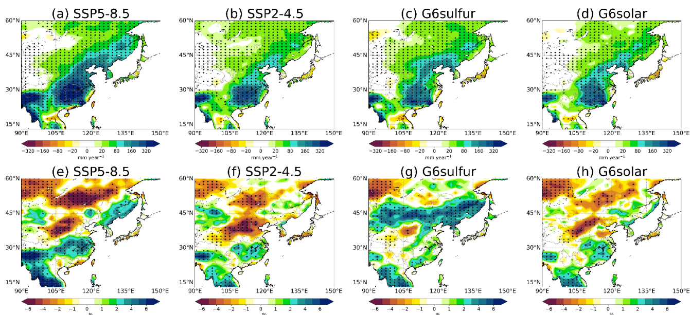
705 Figure 9: Absolute changes in the annual accumulation of AR-related precipitation (a-d) and the fractional contribution of ARs to annual total precipitation amount (e-h) for the future period (2071-2100) relative to the historical baseline (1981-2010). Stippling indicates changes that are statistically significant at a confidence level of > 95% (p-value < 0.05 based on the Student's t-test).
