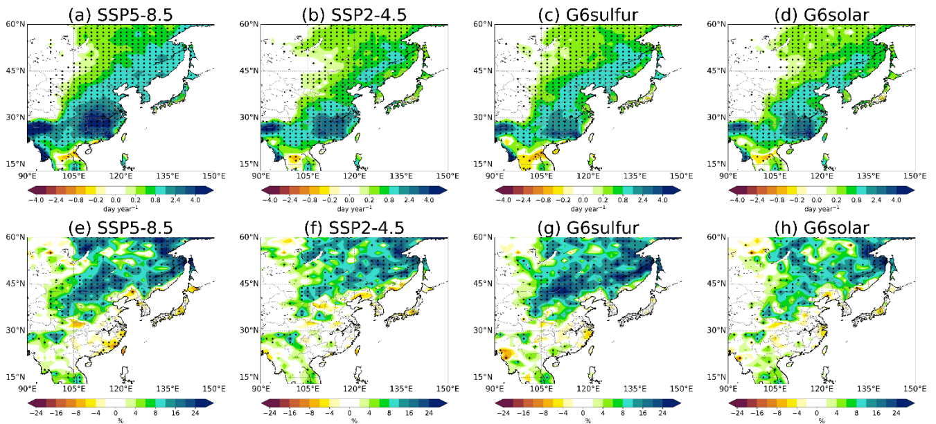
710 Figure 10: As Figure 9, but for the occurrence of AR-related events (a-d) of heavy rain (daily precipitation > 40 mm) and the contribution of ARs to the annual total heavy rain events (e-h).
