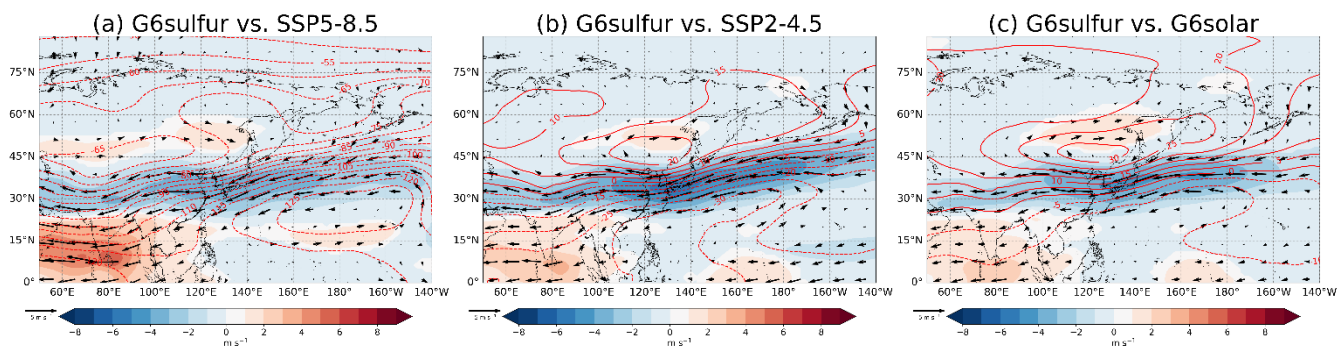
685 Figure 5: Differences in MJJAS-mean geopotential thickness between 200 and 500-hPa (red contours) and 200-hPa winds (shaded for velocity and vectors for direction) for the future period of 2071-2100 between G6sulfur and SSP5-8.5 (a), SSP2-4.5 (b) and G6solar (c).
