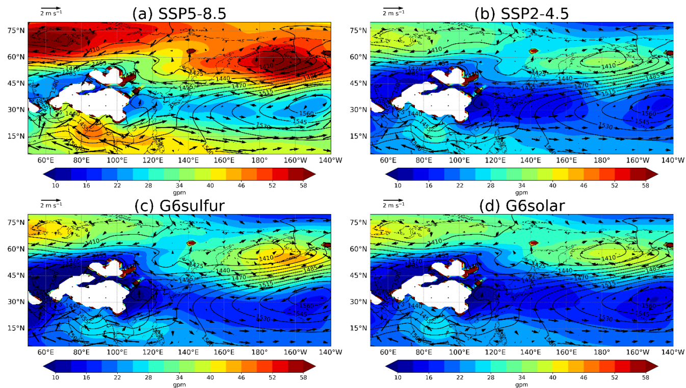
665 Figure 1: Absolute changes in MJJAS-mean geopotential height (shaded, unit: geopotential meter / gpm) and winds (vectors) at 850-hPa for the future period of 2071-2100 relative to the historical baseline during 1981-2010. Black contours show the MJJAS-mean 850-hPa geopotential height during the historical baseline period. Areas with a surface pressure below the 850 hPa level are shown in white.
