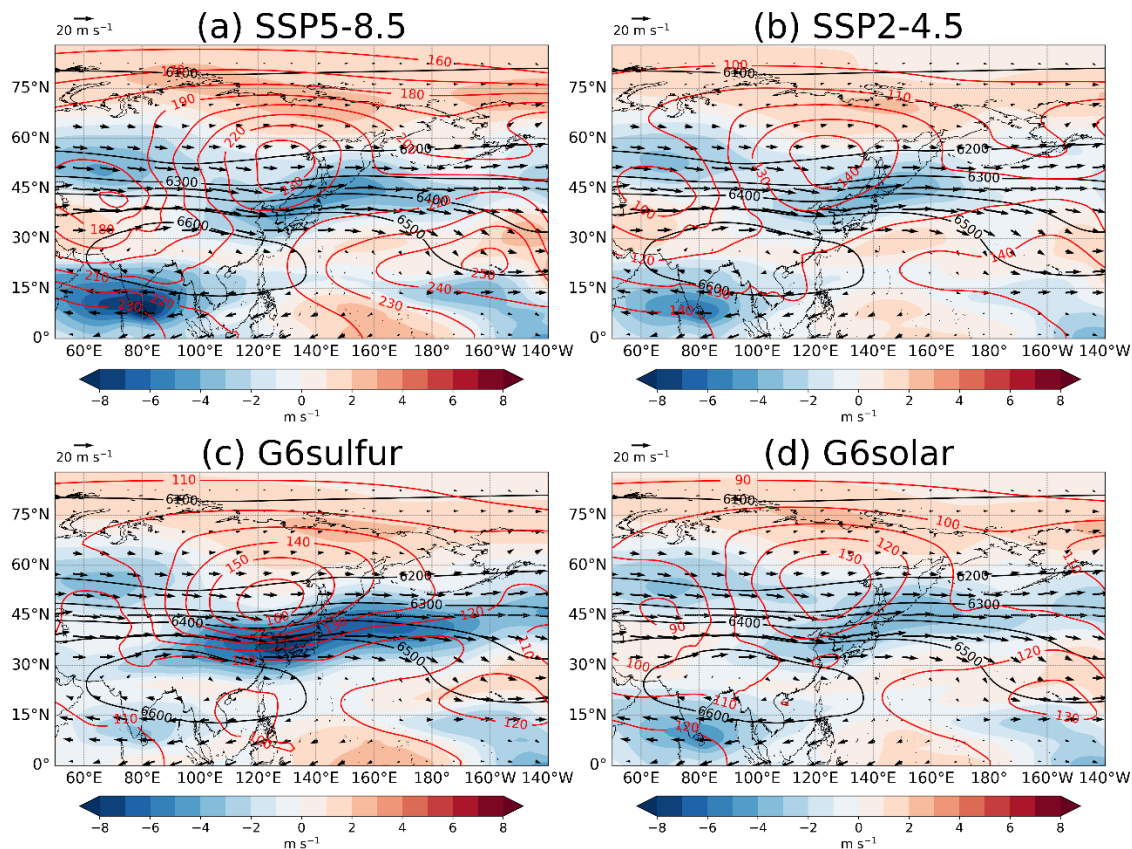
680 Figure 4: Absolute changes in MJJAS-mean geopotential thickness between 200 and 500-hPa (red contours, unit: gpm) and 200-hPa wind speeds (shaded) for the future period of 2071-2100 relative to the historical baseline during 1981-2010. Black contours (unit: gpm) show the MJJAS-mean 200-500-hPa geopotential thickness and vectors show the MJJAS-mean 200-hPa wind fields during the historical baseline period.
