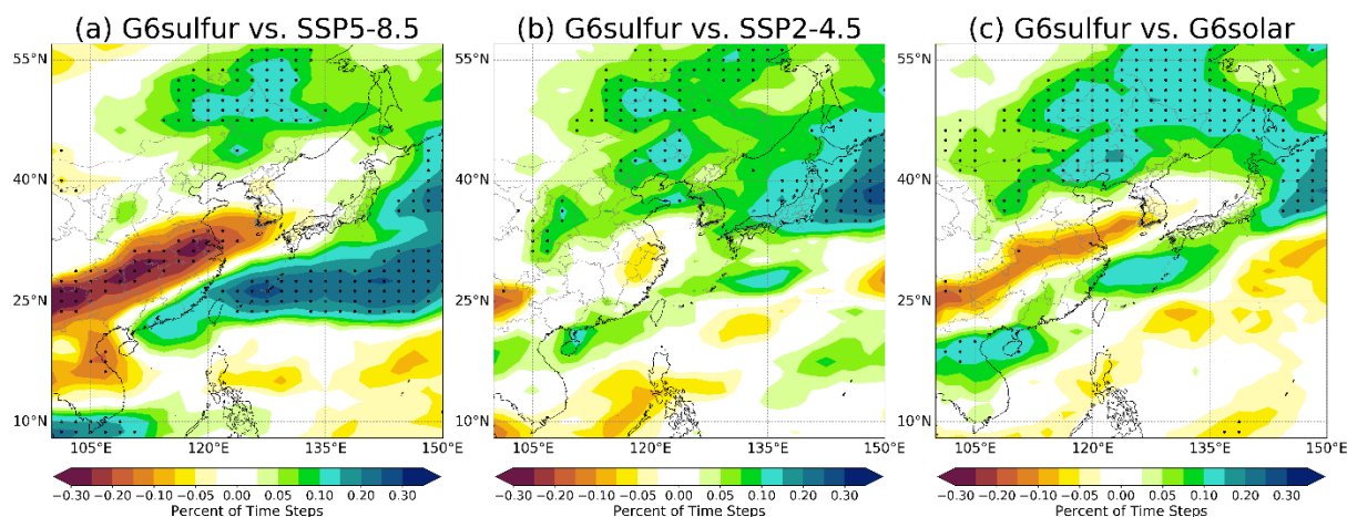
700 Figure 8: Differences in annual mean AR frequency for the future period of 2071-2100 between G6sulfur and SSP5-8.5 (a), SSP2-4.5 (b) and G6solar (c). Stippling indicates differences that are statistically significant at a confidence level of > 95% (p-value < 0.05 based on the Student's t-test).
