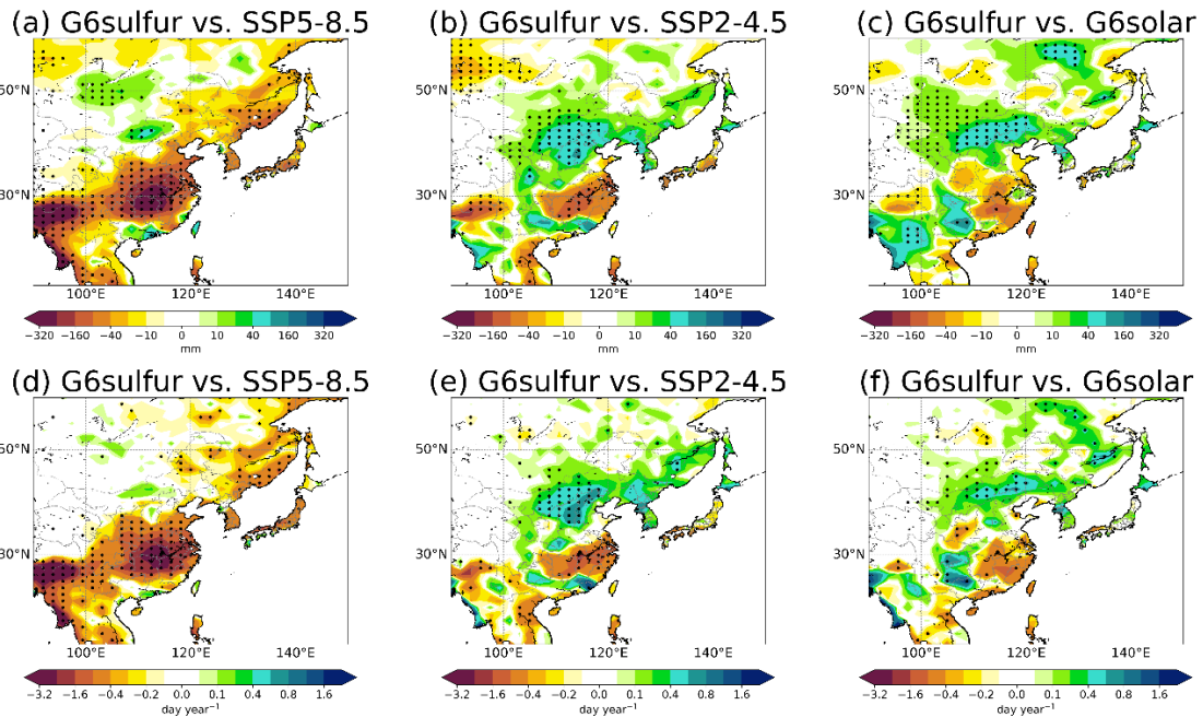
715 Figure 11: Differences in annual accumulation of AR-related precipitation (a-c) and heavy rain events (d-f) for the future period of 2071-2100 between G6sulfur and SSP5-8.5 (a, d), SSP2-4.5 (b, e) and G6solar (c, f). Stippling indicates differences that are statistically significant at a confidence level > 95% (p-value < 0.05 based on the Student's t-test).
