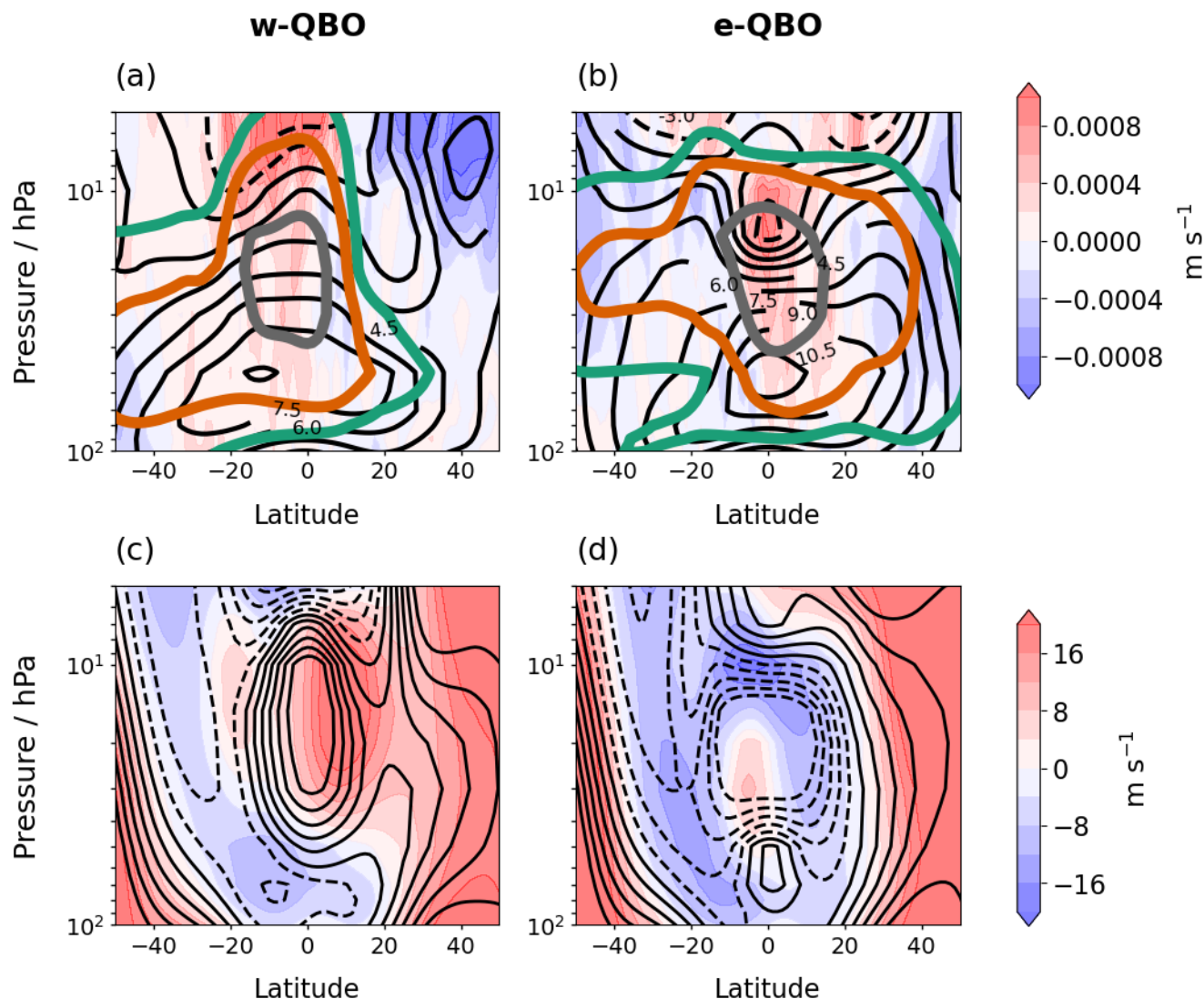
520 Figure 10: Five months after 60 Tg eruptions in July: (a), (b) shows the w anomalies (filled contours), positive temperature anomalies (black solid contours) and sulfate mass mixing ratio anomalies (coloured contours) with respect to the control ensemble mean. The sulfate mass mixing ratio contours are at interval of 5 \times 10^{-8} , 15 \times 10^{-8} , 50 \times 10^{-8} \text{ kg kg}^{-1} and the temperature contours are in intervals of 1.5 K. (c), (d) The monthly mean zonal wind after the eruption (filled contours) compared to the control (black contours). The filled contour intervals are the same as the line contours, with dashed lines representing negative zonal winds in the line contours. 525 Panels (a) and (c) show results for the w-QBO, and panels (b) and (d), for the e-QBO.
