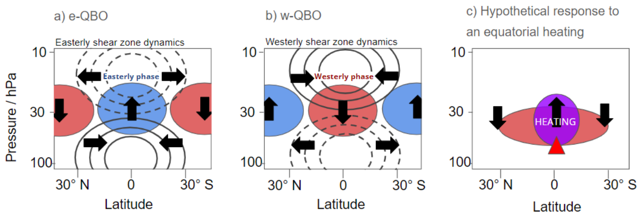
230 Figure 1: Schematic temperature and circulation anomalies (a) associated with a lower stratospheric easterly shear zone and upper stratospheric westerly shear zone, (b) associated with a lower stratospheric westerly shear zone and upper stratospheric easterly shear zone, and (c) in response to heating from a volcanic SO 2 injection at the equator at the location indicated with a red triangle. Panels (a) and (b) are adapted from Plumb and Bell (1982). The black line contours in (a) and (b) represent positive and negative zonal winds in solid and dashed lines, respectively. Positive temperature anomalies (filled shading) are shown in red and negative temperature anomalies are shown in blue. Arrows indicate circulation anomalies relative to the climatological average. The purple circle in panel (c) indicates the heating rate anomaly from the volcanic sulfate, which is narrow compared to the temperature anomaly. 235
