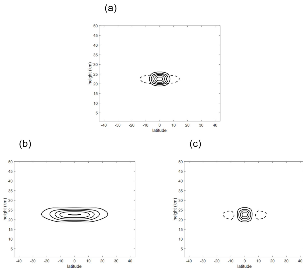
Figure 6: (a) Applied heating field Q_{volc} (solid contours) and Q_{volc} - w \kappa T_b / H (dashed contours). Contour interval is 10^{-6} \text{ K s}^{-1} . (b) Temperature response to applied heating, averaged over the 1 year period for which the heating is applied. Contour interval is 0.5 K. (c) Corresponding response in vertical velocity. Contour interval is 10^{-4} \text{ m s}^{-1} , positive contours solid, negative contours dashed, zero contour not shown.
