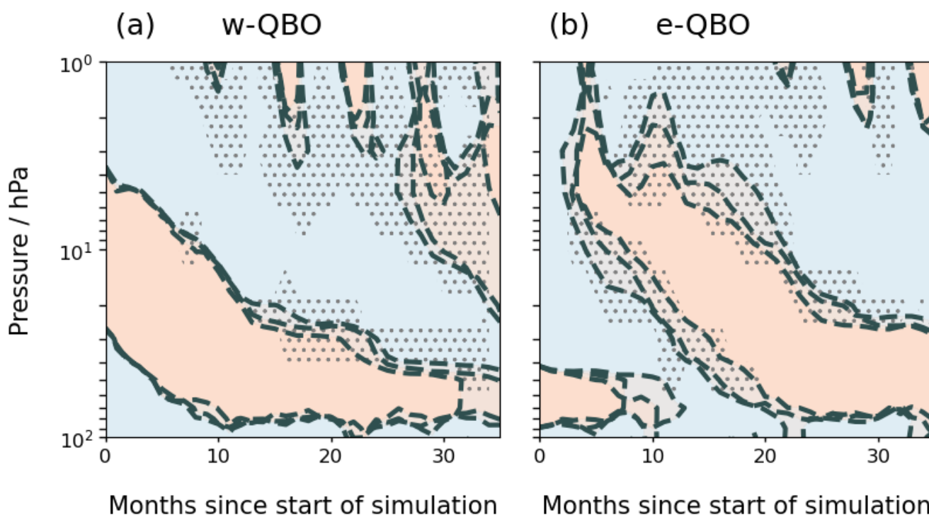
300 Figure 2: Mean zonal wind direction averaged 2° N–2° S for all control ensemble member simulations initiated during (a) a w-QBO and (b) an e-QBO. Dashed lines indicate the zero-wind line for each ensemble member, orange shading indicates positive zonal wind, blue indicates negative zonal winds. Stippling occurs where the standard deviation of the zonal wind across control ensemble members is greater than 4 m s -1 .
