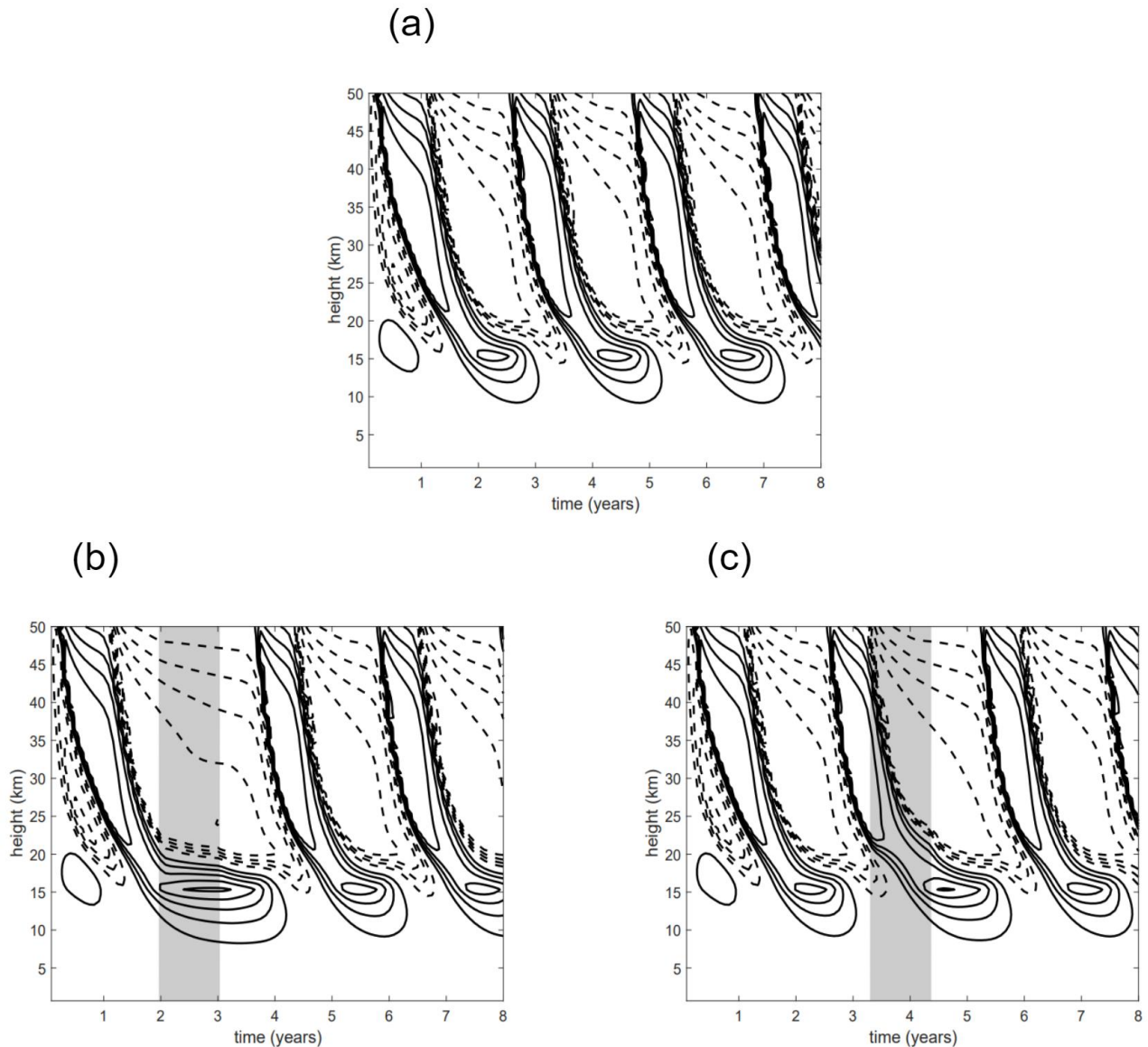
425 Figure 7: (a) Evolution of u at equator in control experiment. Contour interval is 2.5 \text{ m s}^{-1} , positive contours solid, negative contours dashed, zero contour not shown. (b) Evolution of u when heating is applied for months 25–36 of the simulation, (i.e., an e-QBO 430 configuration). These months are indicated by shading. (c) Evolution of u when heating is applied for months 41–52 of the simulation (a w-QBO configuration).
