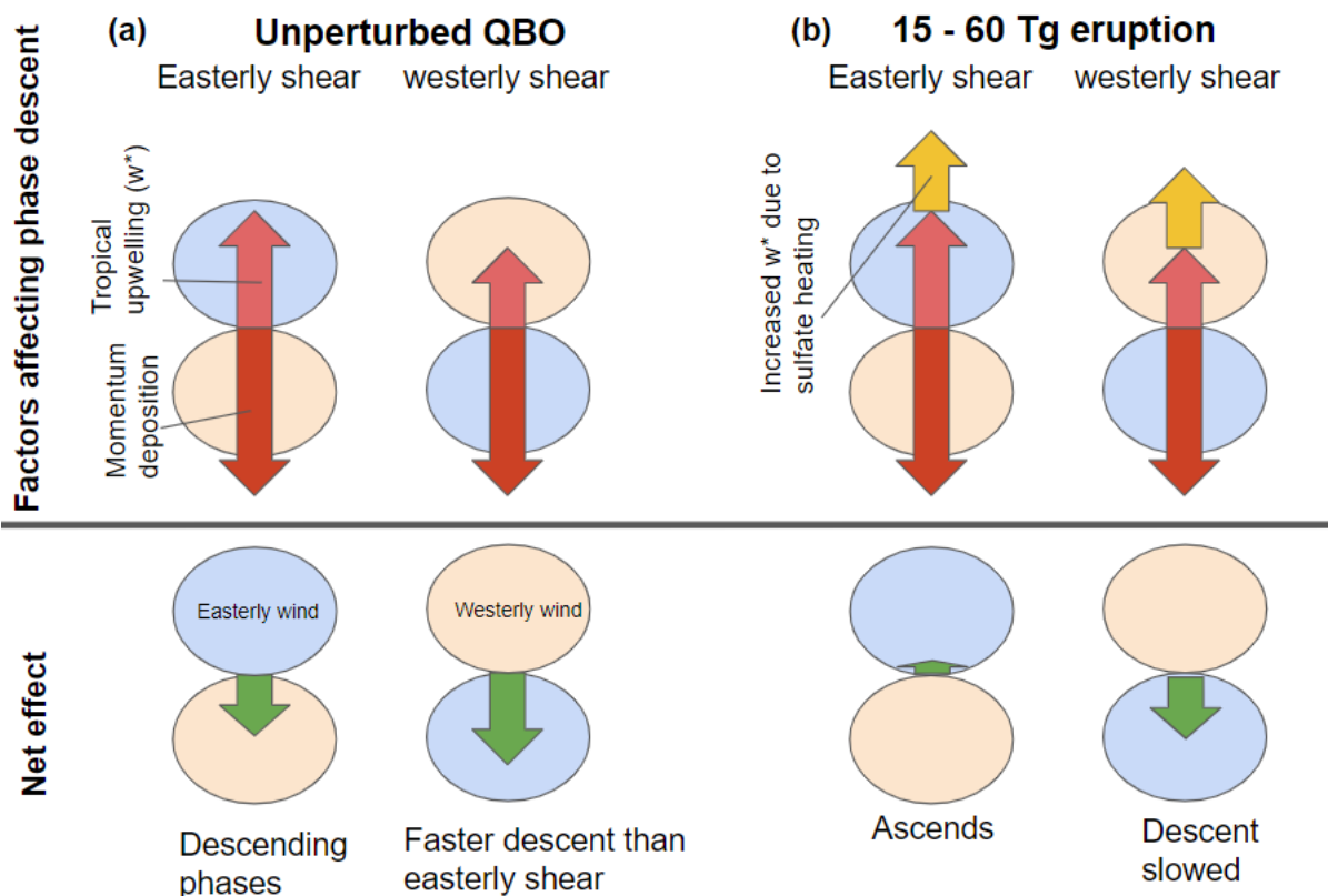
620 Figure 11: Schematic representing (top row) the most important factors controlling the QBO momentum balance and (bottom row) the net effect of these factors on the easterly shear descent rate and the westerly shear descent rate during (a) an unperturbed QBO and (b) a Tambora-magnitude or Pinatubo-magnitude eruption simulated in the tropics. Arrows indicate the effect on the movement of the QBO phases due to mean vertical advection of zonal momentum, w \frac{\partial u}{\partial z} (pink), momentum deposition (red), the change in w \frac{\partial u}{\partial z} due to the eruption (yellow) and the net effect of these (green).
