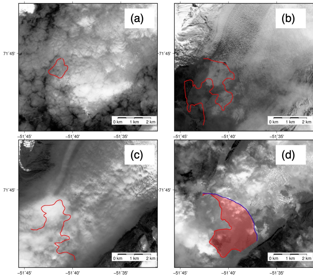
Figure 5. Examples of results abandoned for different reasons. (a) Short terminus. (b) & (c) Long and complex terminus. (d) Terminus forms a large polygon with its adjacent picks. The backgrounds are the source images of the wrong picks. The red line in (d) is the wrong pick and the blue curve shows its time-adjacent manual pick.
