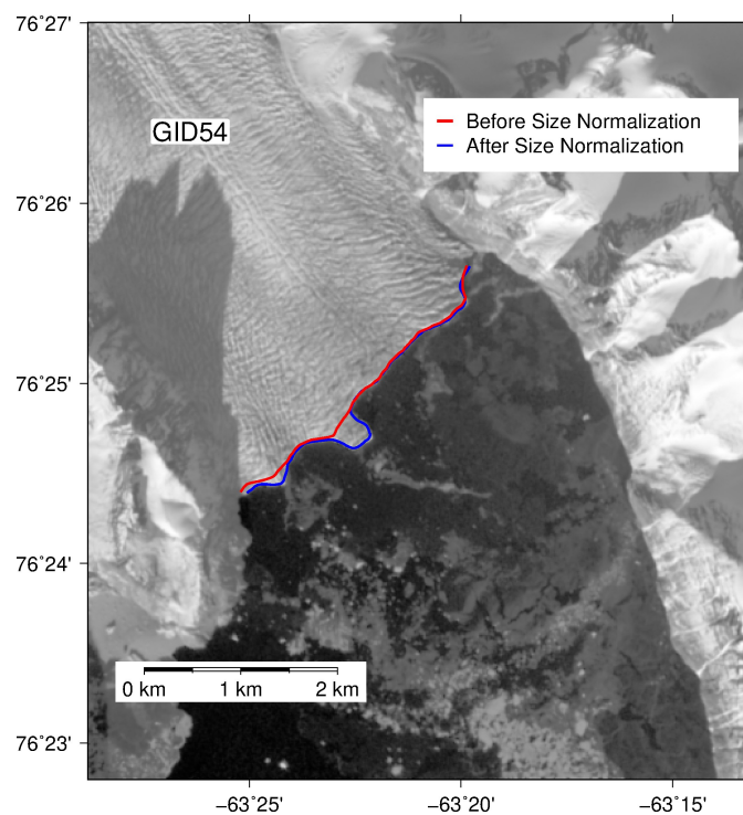
Figure 13. An example showing the effect of size normalization for Glacier ID #54. After normalization, delineation of the terminus is more accurate and captures small features.
