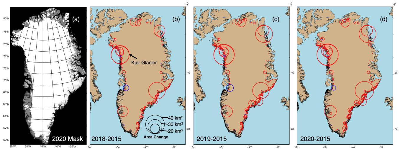
Figure 12. An example of an updated ice mask for 2020 (a) and the terminus change between the updated masks and the original 2015 GrIMP ice mask (b–d; 2018–2020). Red circles represent retreating glaciers and blue circles represent advancing glaciers. The size of the circle indicates the difference in area change of each glacier from the original mask. The boundary of the GrIS in (b–d) is the same with Fig. 7, provided by GMT.
