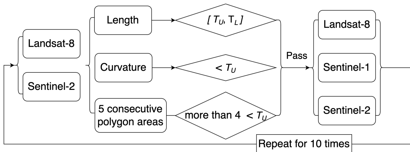
Figure 3. The pipeline of the screening module. T_U is the upper threshold and T_L is the lower threshold. Each metric (length, curvature, 5-consecutive areas) has its own threshold. Only the results from optical images are used to calculate the thresholds, and the thresholds are applied uniformly to all the datasets.
