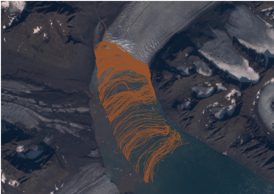
Figure R6. Glacier termini of GID144.
