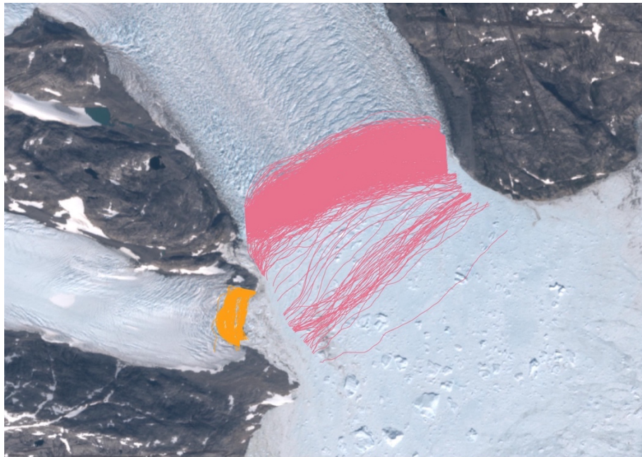
Figure R10. Glacier termini of GID210 (pink) and GID211(orange).
