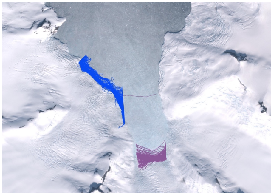
Figure R11. Glacier termini of GID214 (blue) and GID215(purple).
