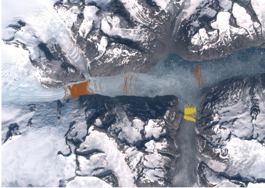
Figure R12. Glacier termini of GID253 (brown) and GID254(yellow).
