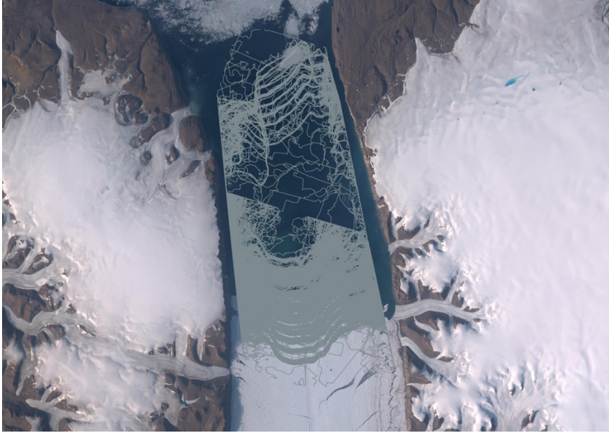
Figure R5. Glacier termini of GID86.
