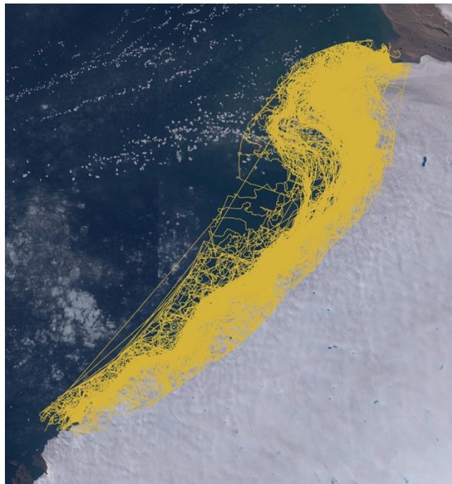
Figure R3. Glacier termini of GID85.
