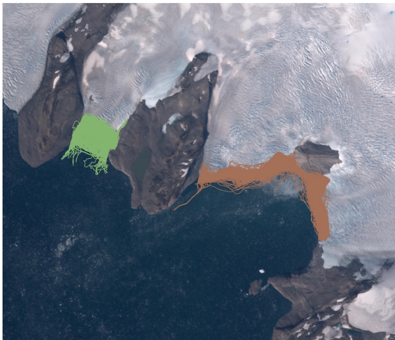
Figure R4. Glacier termini of GID44 (brown) and GID45 (green).
