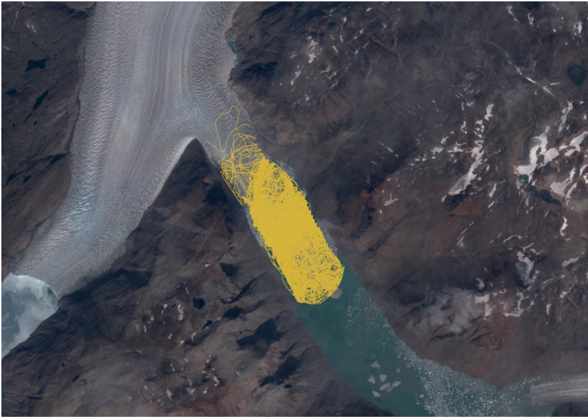
Figure R13. Glacier termini of GID262.
