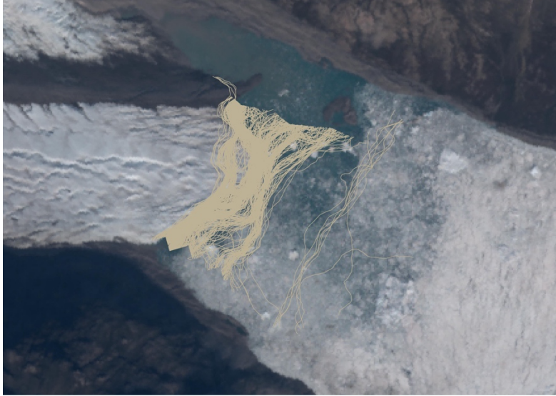
Figure R7. Glacier termini of GID120.
