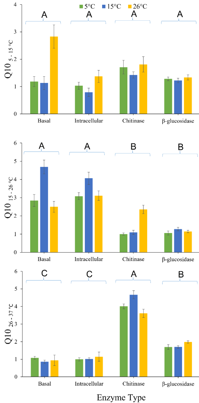
Figure 3: Effects of pre-incubation temperature on temperature sensitivity (Q10 5-15°C , Q10 15-26°C , and Q10 26-37°C ) of basal respiration rate, glucose-induced respiration, and extracellular (chitinase and β-glucosidase) enzyme activity. Each bar and error bar represent mean and standard error of 4 replicate samples each pre-incubated at one of three different pre-incubation temperatures (5 °C, 15 °C, or 26 °C). Assay types sharing the same upper case letters are not significantly different ( P > 0.05 ).
