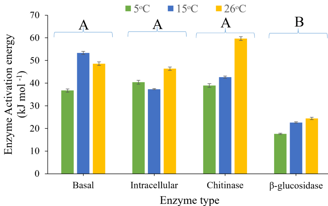
615 Figure 4: Effects of pre-incubation temperature (5 °C, 15 °C, or 26 °C) on Arrhenius enzyme activation energy (E a ) for basal respiration rate, intracellular (glucose substrate induced respiration) enzyme activity, and extracellular (chitinase and β-glucosidase) enzyme activity. E a was calculated for two ranges of temperature (5 °C – 26 °C for intracellular enzymes and basal respiration, and 5 °C – 37 °C for the two extracellular enzymes). Each bar and error bar represent mean and standard error of 4 replicates. Enzyme types sharing the same upper case letters are not significantly different ( P > 0.05 ).
