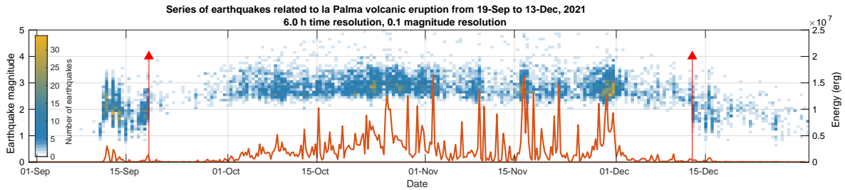
Figure 14. Seismic activity associated with the La Palma volcano eruption for the whole period, showing in colors the histogram of magnitudes and the integrated generated seismic energy with an orange line. The red arrows mark the start and end of the volcanic eruption.
