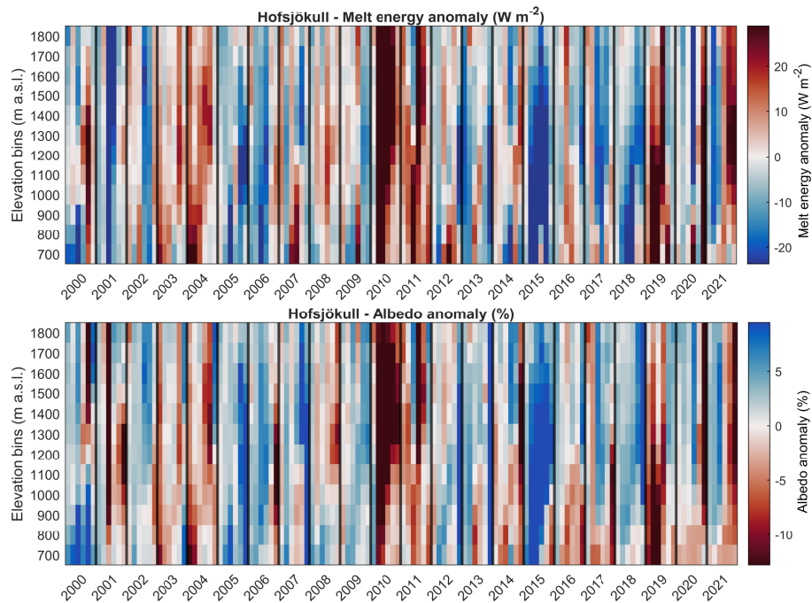
Figure B2. Distribution of melt energy and albedo anomalies ( \text{W m}^{-2} ) with elevation for Hofsjökull. Vertical axis shows elevation bins in 100 m intervals and horizontal axis shows monthly data for each year from April to September. Black vertical lines separate.
