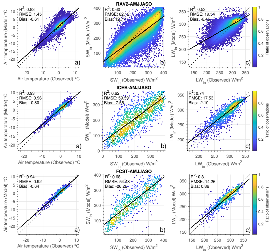
Figure 2. Comparison of the downscaled daily model forcings, 2 m air temperature (a), incoming solar radiation (SW ↓ ) (b) and incoming long-wave radiation (LW ↓ ) (c), with ground observations from the GAWS network. Data is shown for averages from April through October (AMJJASO). Color shows the normalized (0–1) density distribution of data. Different rows indicate different data sources (RAV2, ICEB and FCST) used in the comparison, see Section 3.3. Dotted black line shows 1:1 and black line the calculated linear fit to the data. Further details are in Table 2.
