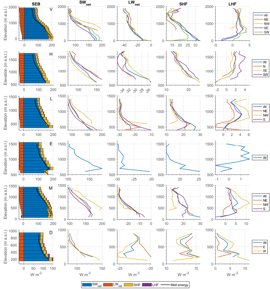
Figure 4. Variation of surface energy balance components with elevation (100 m elevation bins). The first column of images shows the average MJJA energy balance by elevation for the whole glaciers. The other columns show individual SEB components for the glaciers and their main sub-areas as a function of elevation. (Sub-areas are defined in Fig. 1). V: Vatnajökull; H: Hofsjökull; L: Langjökull; E: Eyjafjallajökull; M: Mýrdalsjökull; D: Drangajökull. Note that the horizontal scale varies between panels. SW_{net} is the incoming short-wave radiation, LW_{net} is the net long-wave radiation, SHF is the sensible heat flux and LHF the latent heat flux.
