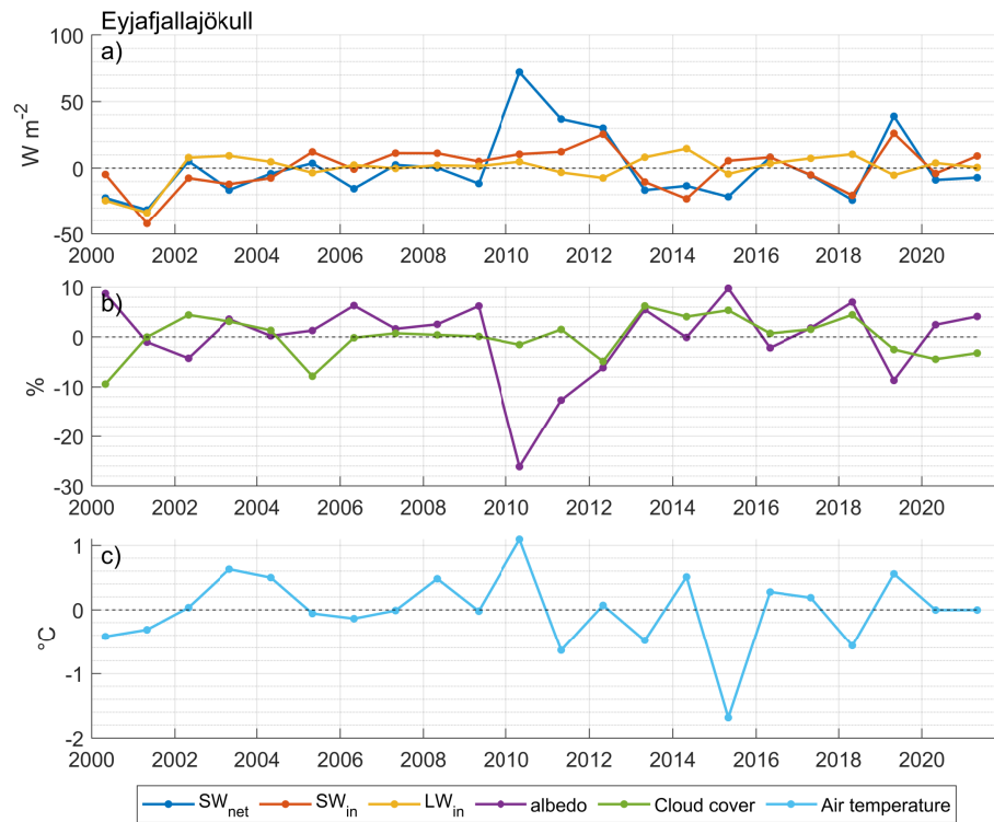
Figure B10. Annual anomalies (MJJA) for selected variables for Eyjafjallajökull. a) net short-wave radiation ( SW_{net} ), incoming short-wave radiation ( SW \downarrow ) and incoming long-wave radiation ( LW \downarrow ), b) albedo and cloud cover and c) 2 m air temperature.)
