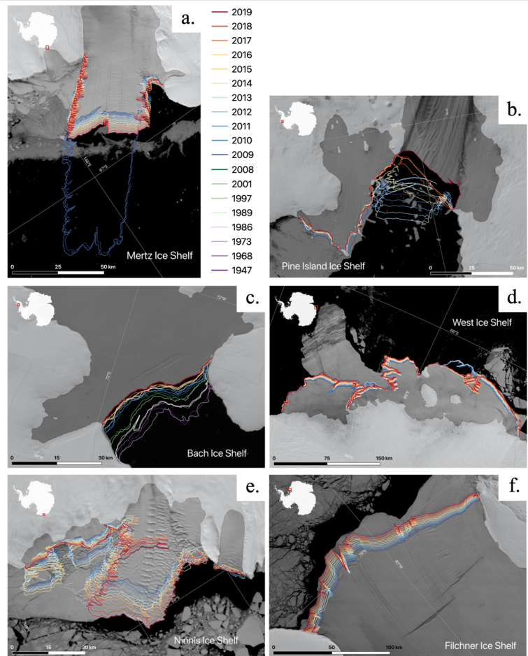
Figure 2: Maps of calving front change from 1947-2019 representing a. a major calving event b. rapid calving front retreat, c. gradual calving front retreat, d. advance with periodic retreat, e. rapid calving front advance and f. steady calving front advance overlaying MODIS satellite images from 2019 (Scambos et al., 1996).
