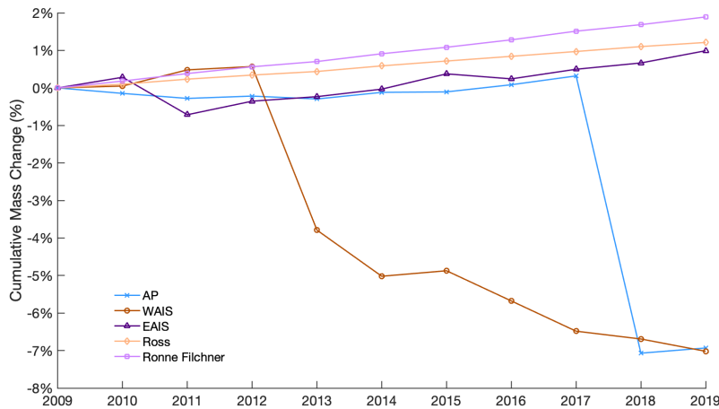
Figure 4. Cumulative ice shelf mass change from 2009 to 2019 for the AP, WAIS, EAIS, Ross Ice Shelf, and Ronne Filchner Ice Shelves.
