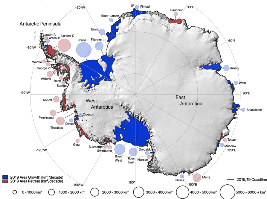
105 Figure 1: Antarctic map of ice shelf area change from 2009 to 2019 with ice shelf names overlaid on a Bedmap2 surface of Antarctica. Circle areas denote total amount of ice shelf area in km 2 lost (red) or gained (blue). The black bold line represents the Antarctic coastline, combining 2015 and 2019 data.
