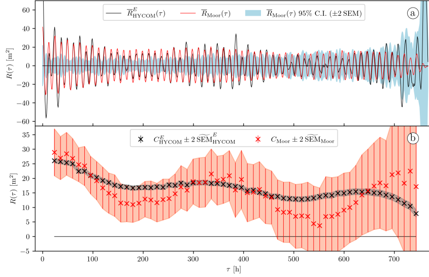
Figure 4. (a) Mean autocovariance computed from \eta_{1000}^E (solid black curve, same as the solid red curve in Fig. 3a ), and mean autocovariance computed from eleven 32-day segments of the mooring No. 2 time series (solid red curve) and 95% confidence interval of \bar{R}_{\text{Moor}} (light blue shading) . (b) Complex demodulates at the semidiurnal frequency of the autocovariance series shown in (a) and their 95% C.I. The red and grey shadings highlight the 95% C.I. for the mooring and Eulerian HYCOM data, respectively.
