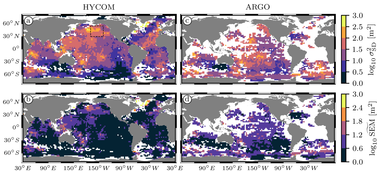
Figure 6. (a) Atlas of the total semidiurnal IT variance computed as the first 48-h complex demodulate of the local mean autocovariance series at 1,000 dbar ( \bar{R}_{\text{HYCOM}}^L ), and (b) corresponding total error computed from Eq SEM. (??). (c) and (d) Same as (a) and (b), respectively, but computed from the Argo data ( \bar{R}_{\text{Argo}} ). (c) and (d) are updated from Geoffroy and Nycander (2022). The area where the simulation is affected by the TBI is shown by the dashed black rectangle in (a).
