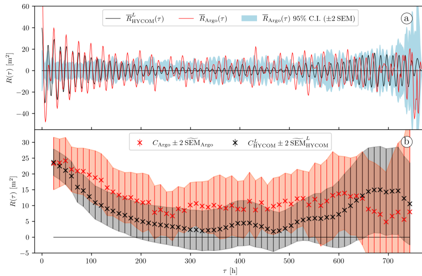
Figure 2. (a) Local mean autocovariance \bar{R}_{\text{HYCOM}}^L computed from the HYCOM particles (solid black curve), and local mean autocovariance \bar{R}_{\text{Argo}} computed from the 32-day segments of Argo data (solid red curve) and 95% confidence interval of \bar{R}_{\text{Argo}} (light blue shading). The data are from the geographical patch shown in Fig. 1. The Argo variance lies above the figure scale, here \bar{R}_{\text{Argo}}(0) \simeq 121 \text{ m}^2 . (b) Complex demodulates at the semidiurnal frequency of the autocovariance series shown in (a) and their 95% C.I. The red and grey shadings highlight the 95% C.I. for the Argo and Lagrangian HYCOM data, respectively.
