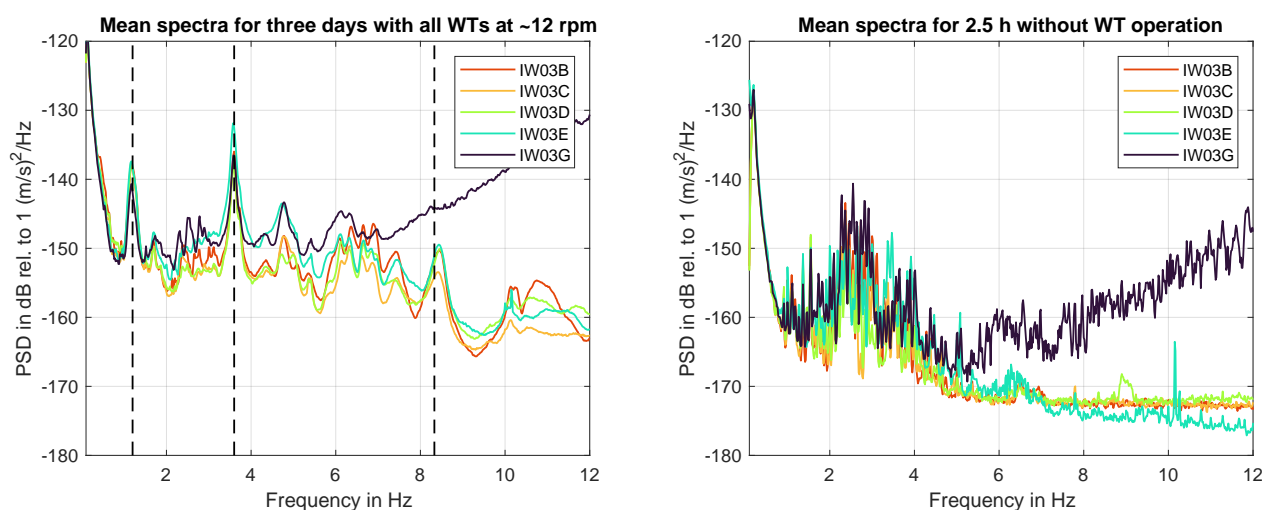
Figure 14. Spectra for amplitude decay estimation for wind farm Lauterstein with 16 WTs. Left: Mean spectra for instruments IW03B-E and IW03G for three days of full operation of the wind farm. Frequencies used for amplitude decay estimation are marked by black-dashed lines. Right: Mean spectra for 2.5 hours without WT operation. The increased PSD levels at site IW03G for frequencies above 5 Hz originate from a nearby gas heating.
