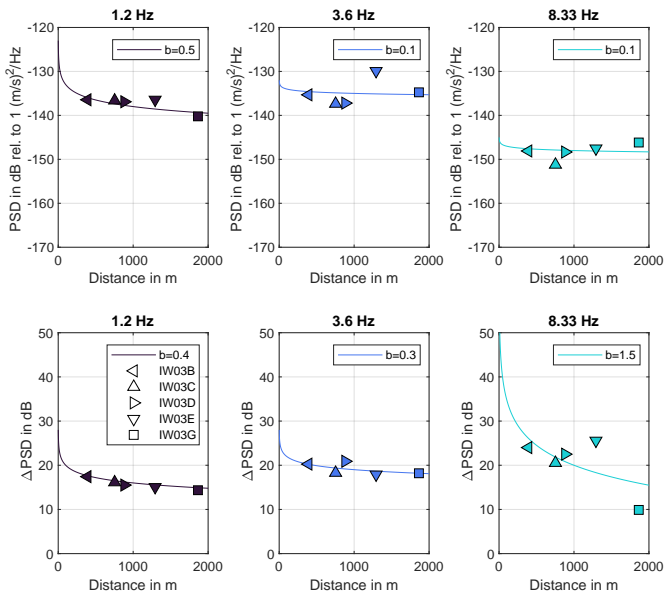
Figure 16. Amplitude decay estimation for full operation at wind farm Lauterstein. Top: amplitude decay for PSD peaks. Bottom: amplitude decay for relative PSD values. The estimated b -values are graphically compared in Figure 17 and are listed in Table 3.
