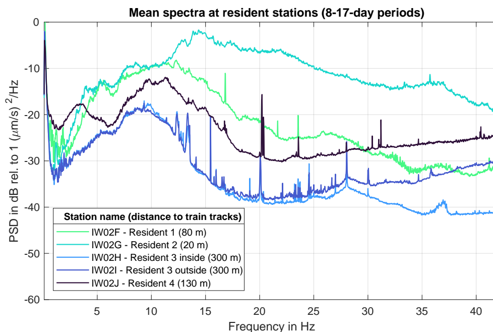
Figure 8. Mean spectra for 8 to 17 day long measurements at residents in the municipality of Kuchen. Amplitude and frequencies excited are closely related to the distance of the measurement location to the train tracks. Two instruments were installed at resident 3, where lower amplitudes are measured in the basement compared to the outside location for frequencies above 25 Hz.
