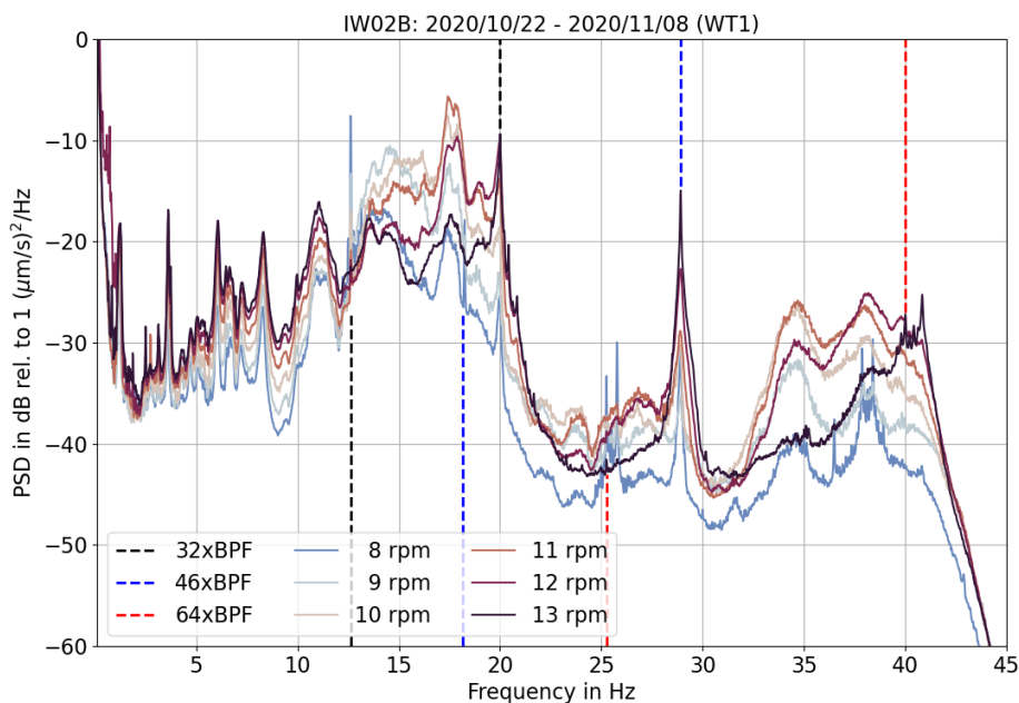
Figure 6. Mean spectra for recording station IW02B (150 m distance to WT 1 of wind farm Tegelberg) for a two week period, sorted by the rotation rate of WT 1. Only spectra for 8 rpm to 13 rpm are shown. Black, blue and red dashed lines mark peaks related to multiples of the BPF for 8 rpm (lines originating at the bottom) and 13 rpm (lines originating at the top), respectively (see Table 2). These frequencies are prominent in the ground motion data and their amplitude distribution relative to wind direction is shown in Figure 7.
