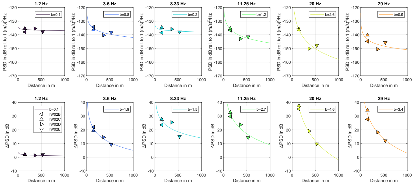
Figure 15. Amplitude decay estimation for full operation at wind farm Tegelberg. Top: amplitude decay for PSD peaks. Bottom: amplitude decay for relative PSD values. The estimated b -values are graphically compared in Figure 17 and are listed in Table 3.
