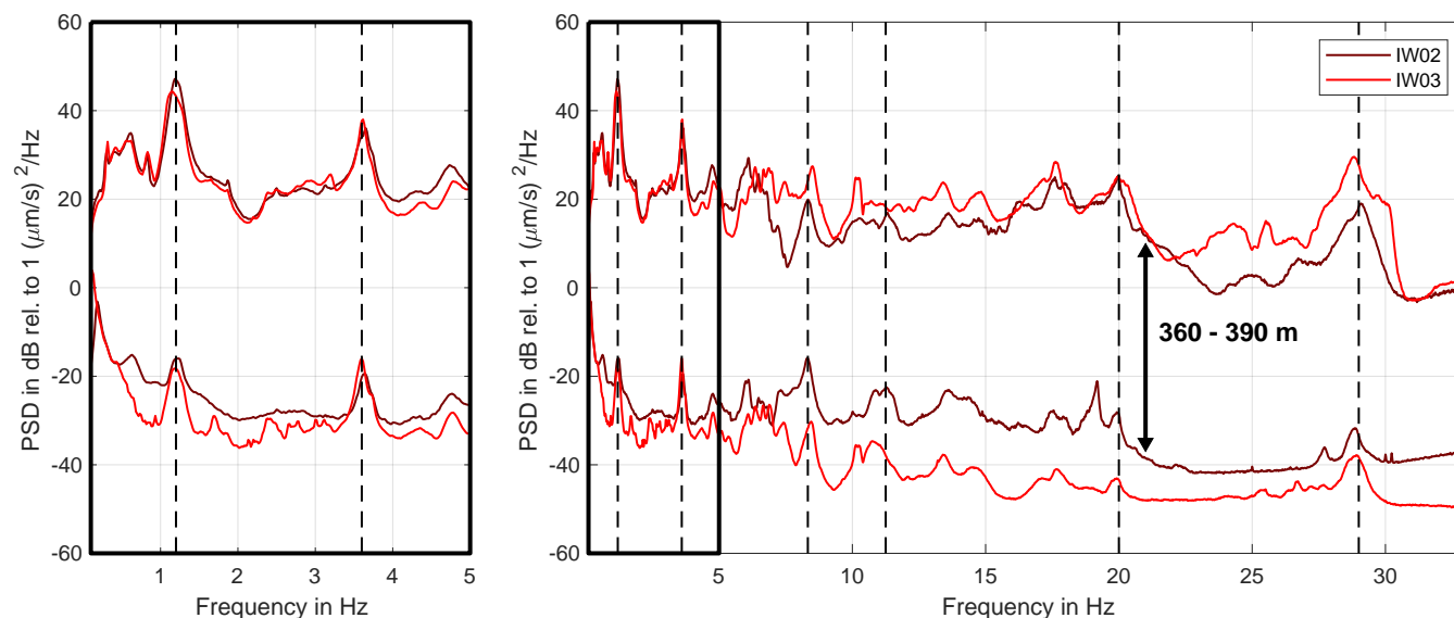
Figure 5. Comparison of mean PSD spectra for recordings inside the WT tower (upper curves) and close by in the free field (lower curves) for measurement campaigns Tegelberg (IW02, dark red, distance 360 m) and Lauterstein (IW03, red, distance 390 m). For Tegelberg all three WT were in full operation for approximately two days. At Lauterstein all 16 WT were in full operation for almost three days. Frequencies considered for amplitude decay analysis are marked by black-dashed lines.
