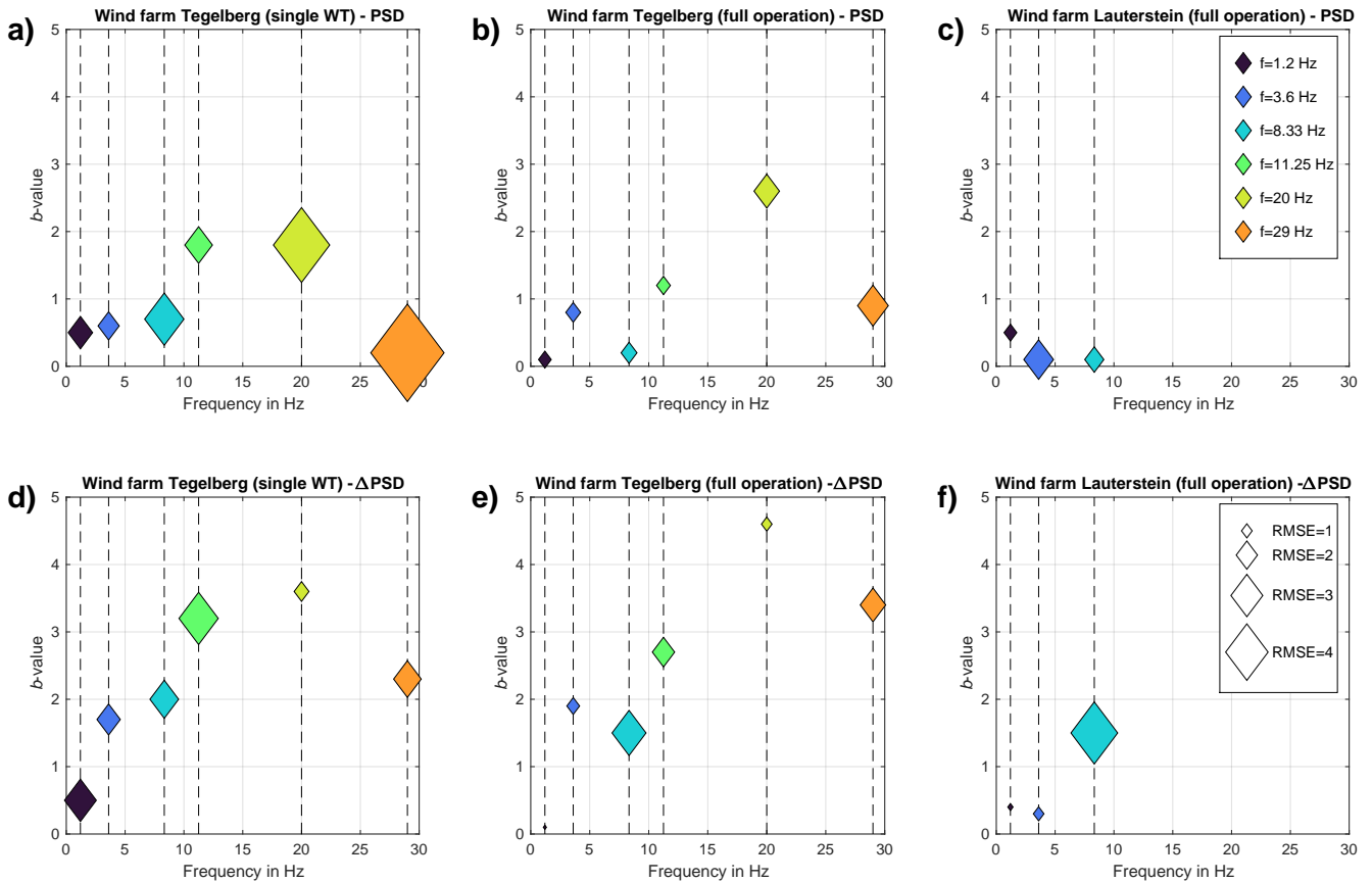
Figure 17. Graphical comparison of b -values for a) and d) single WT operation at wind farm Tegelberg, b) and e) full operation at wind farm Tegelberg, and c) and f) full operation at wind farm Lauterstein. a)-c) b -values for PSD peaks, d)-f) b -values for relative PSD. The size of the symbols corresponds to the RMSE of the measured PSD values compared to the theoretical ones from the fitted curves.
