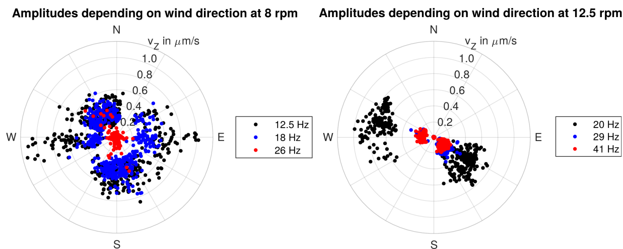
Figure 7. Maximum vertical ground motion amplitudes for 10 min time intervals for the frequencies marked in Figure 6 for station IW02B (150 m distance to WT 1 of wind farm Tegelberg), depending on wind direction, for 8 rpm (left) and 12.5 rpm (right).
