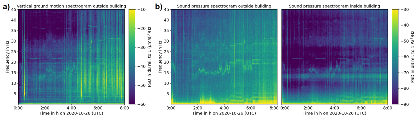
Figure 10. Spectrograms for sites a) IW02F (ground motion), b) IMC_B1 (acoustic indoors) and IMC_B2 (acoustic outdoors) at resident 1 for 2020-10-26 up to 45 Hz. Signals with frequencies 32 \times \text{BPF} can be observed in all three data sets. In the ground motion data train signals dominate before 01:00 UTC and after 03:00 UTC.
