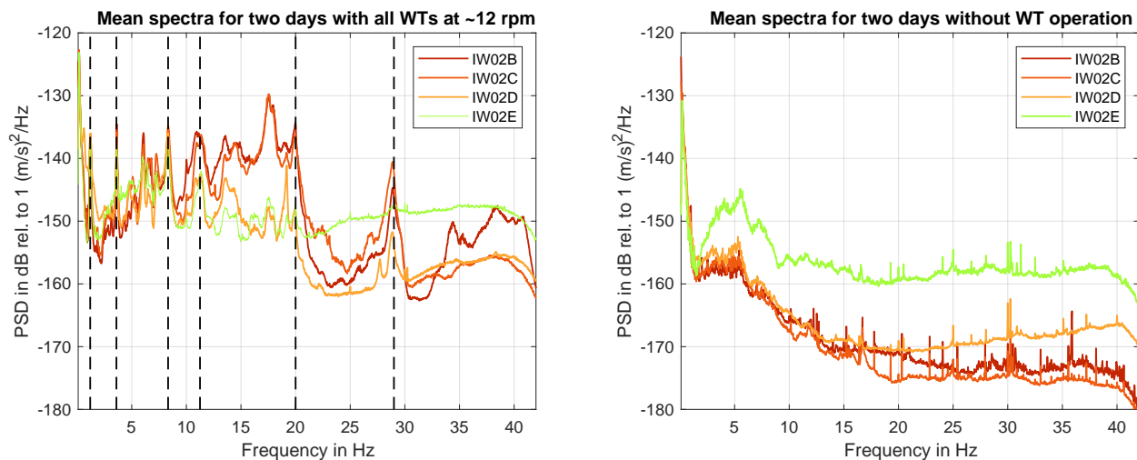
Figure 13. Spectra for amplitude decay estimation for wind farm Tegelberg with three WTs. Left: Mean spectra for sites IW02B-E for two days of full operation of the wind farm. Frequencies used for amplitude decay estimation are marked by black-dashed lines. Right: Mean spectra for two days without WT operation. Note the increased PSD levels at site IW02E which is closest to Kuchen and the railway line.
