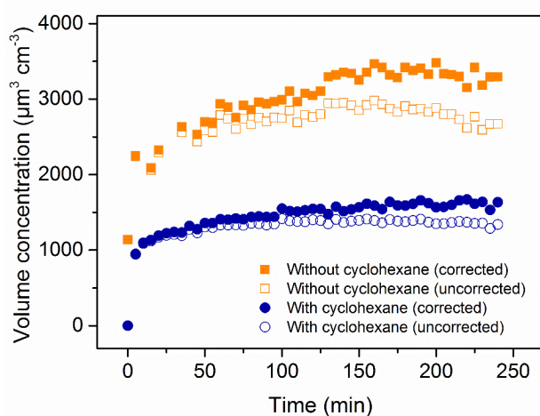
Figure R1. Particle volume concentration as a function of time during the ozonolysis of cyclooctene with and without cyclohexane addition.
