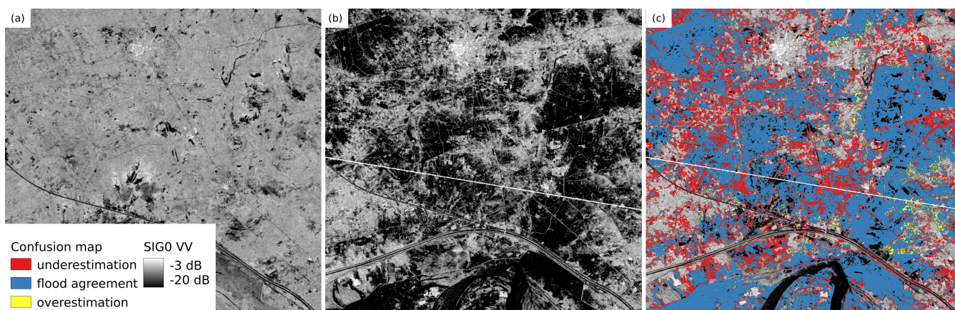
Figure 6. Evaluation for AOI Shikarpur (reference: Copernicus Emergency Management Service (© 2022 European Union), [EMSR629] Shikarpur: Delineation Map, version 1). (a) Expected backscatter from the harmonic model (b) SIG0 VV observation from 2022/08/30 (c) Confusion map
