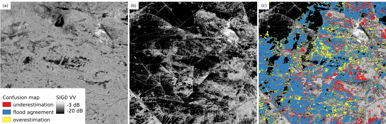
Figure 4. Evaluation for AOI Jacobabad (reference: Copernicus Emergency Management Service (© 2022 European Union), [EMSR629] Jacobabad: Delineation Map, version 1). (a) Expected backscatter from the harmonic model (b) SIG0 VV observation from 2022/08/30 (c) Confusion map
