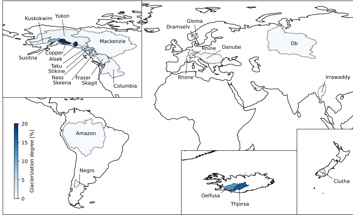
Figure 1. The 25 large-scale (>50,000 km 2 ) glacierized basins for which sufficient runoff observations are found. The hue represents the fraction of basin area covered by glaciers.
