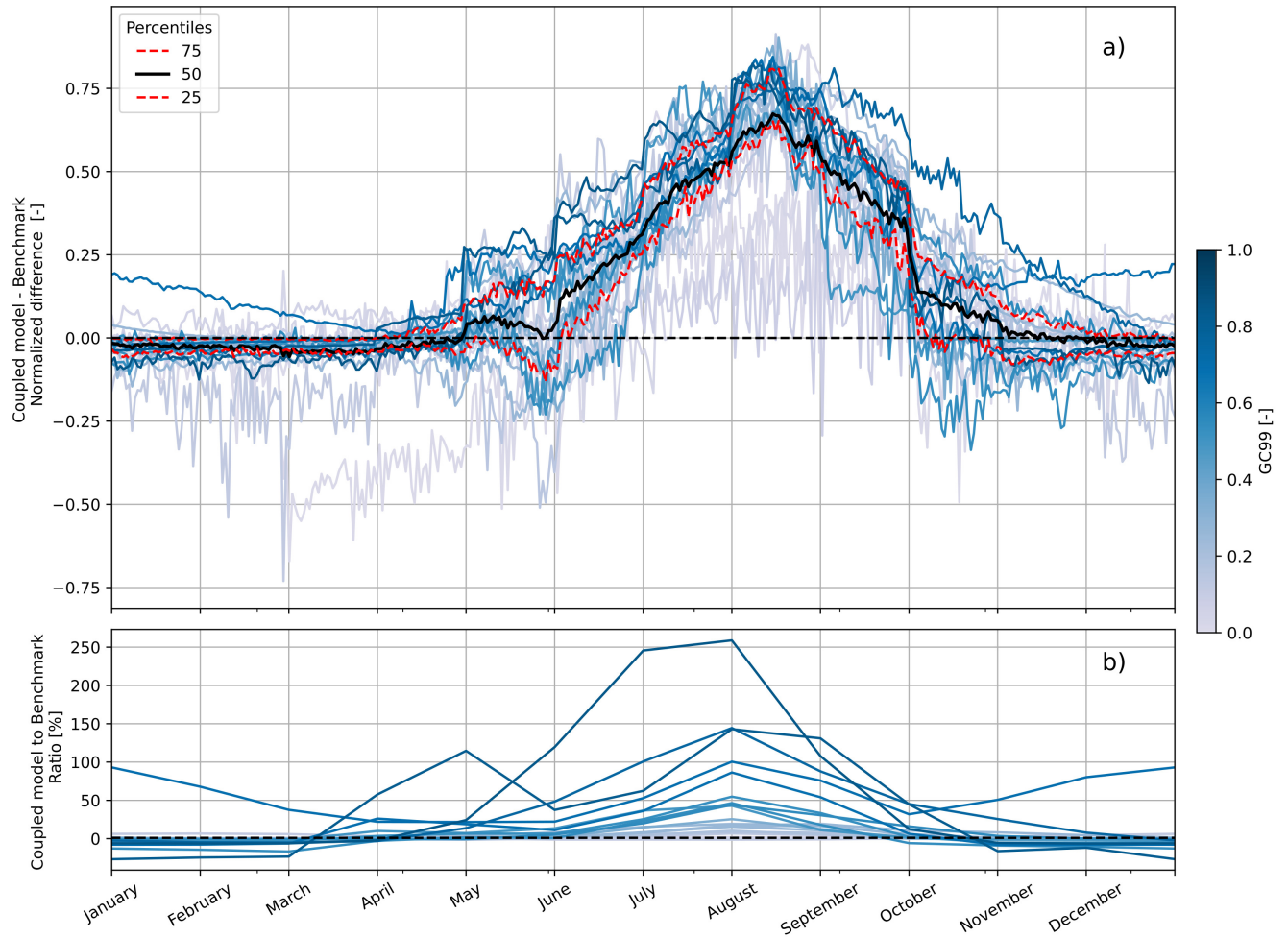
Figure 3. a) Mean normalized difference ( ND ) between the coupled model (PCR GLOBWB 2 & GloGEM) and the benchmark (only PCR-GLOBWB 2) for all 25 basins, showing that the coupled model produces higher runoff estimates throughout the melt season. The normalization is performed against the 99 th percentile of the difference over the whole time range (2001-2012). The mean is computed for each calendar day over the same period. The solid black and dashed red lines represent the quartiles among the 25 basins. b) Ratio of the coupled model to the benchmark, averaged per month and over the period 2001-2012. The blue hue in both figures represents the 99 th percentile of the routed GloGEM glacier runoff contribution to the coupled model runoff (GC99). The data of the three Southern Hemisphere basins are shifted six months forward in time to match the Northern Hemisphere months on the x-axis.
