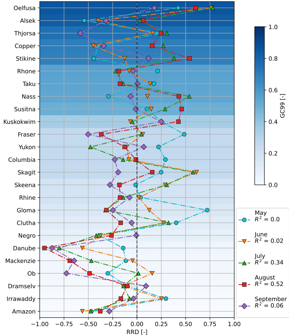
Figure 4. The Relative RMSE Difference ( RRD ) over all 25 basins throughout the melt season. The RMSE difference is calculated relative to the routed glacier runoff, which embodies the maximum possible RMSE difference. Positive scores indicate an improvement of the coupled model over the benchmark compared to observed runoff and vice versa. The RRD always lies between -1 and 1 . The basins are sorted based on the 99 th percentile of the contribution of the routed GloGEM glacier runoff to the coupled model runoff (GC99). The coefficients of determination ( R^2 ) represent the correlation of RRD -scores with the glacier contribution. The months are given only for the Northern Hemisphere, but the results of the three Southern Hemisphere basins are shown for November-March. The distinction between strongly and weakly glacier-influenced basins is set between Sustina and Kuskokwim (GC=0.5).
