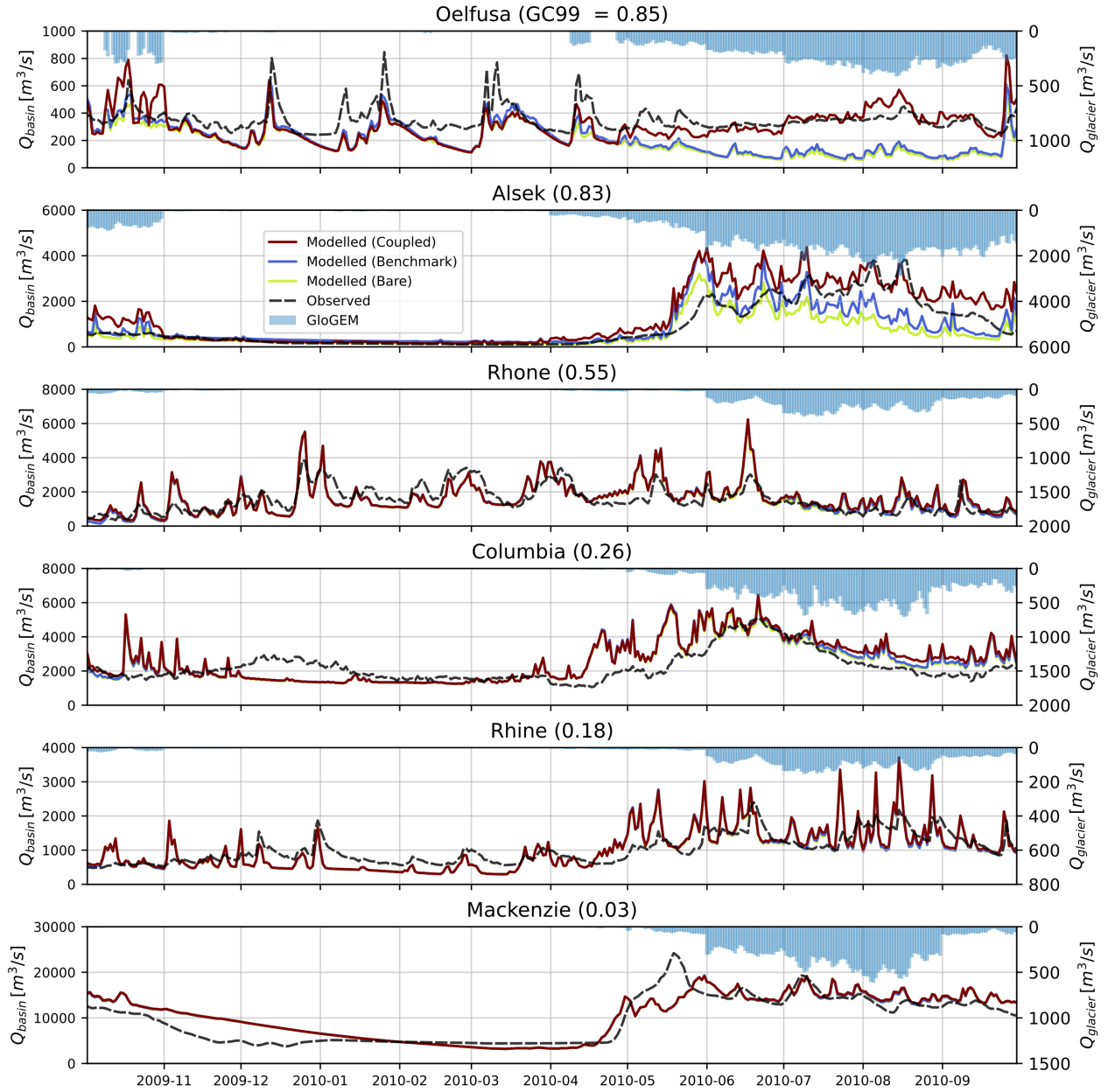
Figure 2. Modelled and observed runoff of a representative selection of the 25 basins for a year close to average conditions. The left y-axis represents the runoff at the selected gauging station, while the right y-axis represents the GloGEM total basin glacier runoff. Note the different extents per basin on the y-axes. The 99th percentile of the GloGEM contribution to the coupled model daily runoff is presented with the basin name. The remaining hydrographs are presented in section 8 of the Supplementary material.
