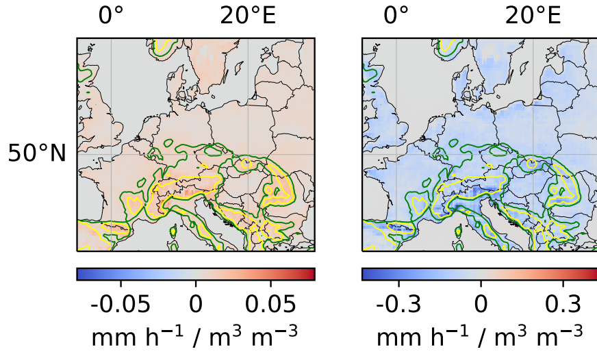
Figure A7. Product of local soil moisture-evaporation and local/ regional evaporation-precipitation couplings. Left: product of local soil moisture-evaporation and local evaporation-precipitation couplings. Right: product of local soil moisture-evaporation and regional evaporation-precipitation couplings. See Appendix Fig. A8 for local soil moisture-evaporation and local and regional evaporation-precipitation couplings.
