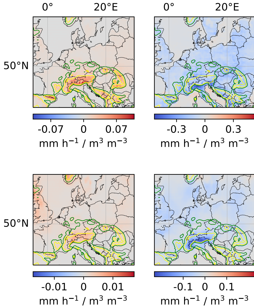
Figure A6. Local and regional soil moisture-convective precipitation and soil moisture-large-scale precipitation couplings. Left column: local couplings. Right column: regional couplings. Upper row: soil moisture-convective precipitation coupling. Lower row: soil moisture-large-scale precipitation coupling.
