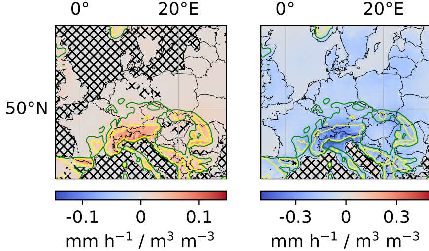
Figure 6. Local and regional soil moisture-precipitation couplings. Left: Impact of local soil moisture changes ( \text{m}^3 \text{ water} \cdot \text{m}^{-3} \text{ soil} ) on local precipitation ( \text{mm h}^{-1} ) for each pixel in the target region (in the text denoted by \overline{q^{loc}_{ij}} ). Right: Impact of local soil moisture changes on regional precipitation for each pixel in the target region (in the text denoted by \overline{q^{reg}_{ij}} ). For better comparability of local and regional values, the unit \text{mm h}^{-1} for precipitation refers to a single pixel in both panels. Missing hatching indicates that the coupling reflects more than random correlations between soil moisture and precipitation in the training data, artifacts of the DL training procedure, seasonality, and the correlation between soil moisture and topography (see Sect. 4.2). The green and yellow elevation contour lines indicate 370 m and 750 m, respectively.
