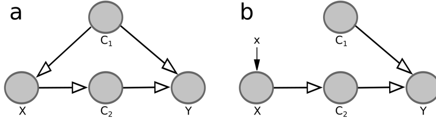
Figure 1. Example for a causal graph (a) and corresponding causal graph for setting variable X to some arbitrary value x (b). The grey circles are referred to as nodes of the graph, while the arrows are referred to as directed edges.
