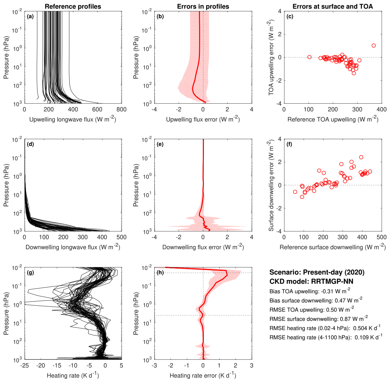
Figure A1. Evaluation of Reduced-RRTMGP-NN longwave fluxes and heating rates using the 50 independent profiles of the CKDMIP Evaluation-1 dataset with present-day concentrations of greenhouse gases. Reference profiles of upwelling, downwelling flux and heating rate from LBL calculations, corresponding errors (b, e, h) with solid lines showing bias and the shaded area giving the 95th percentile of errors, and instantaneous errors in upwelling TOA and downwelling surface fluxes (c, f).
