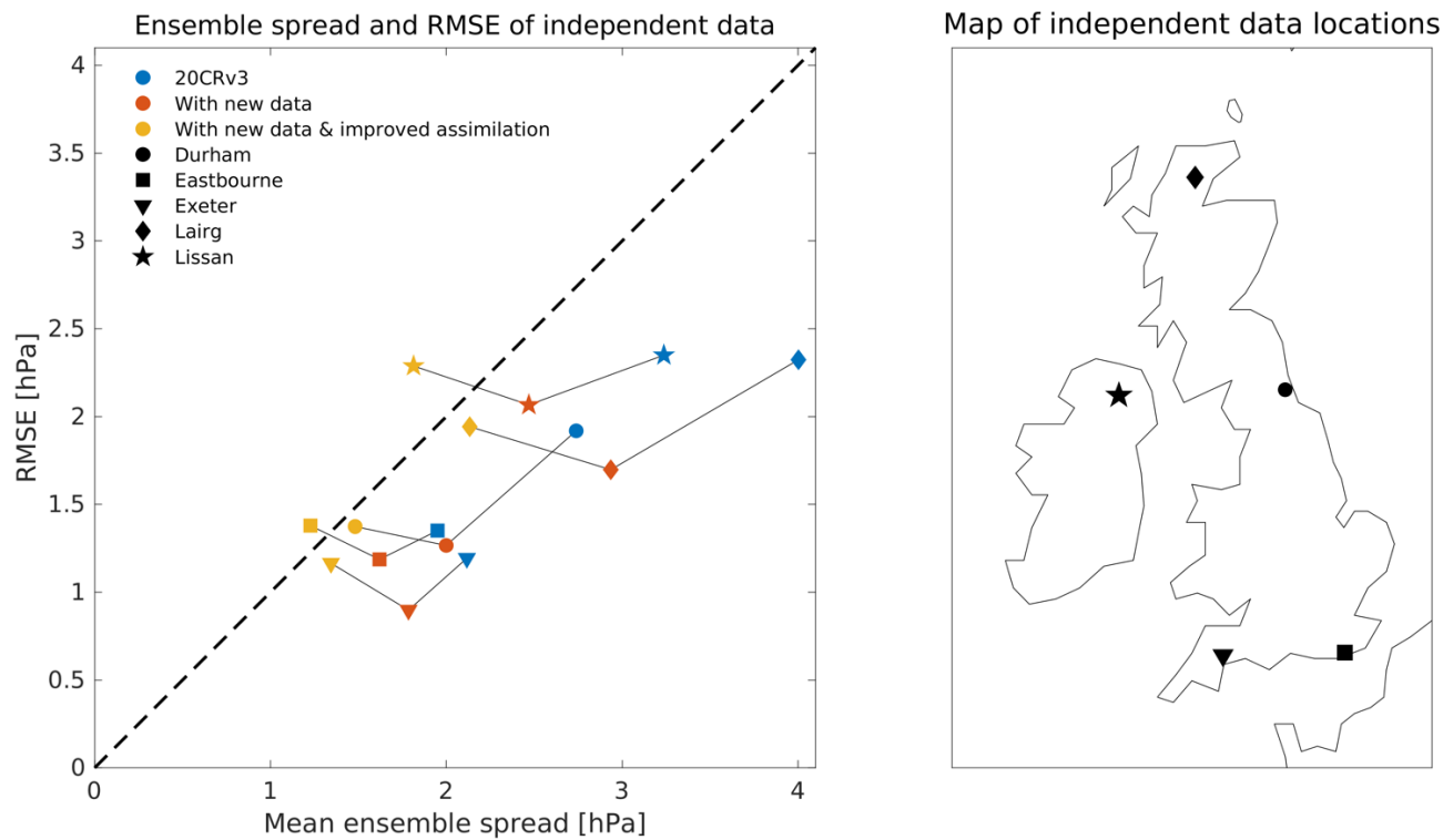
495 Figure B1: Ensemble reliability. Mean ensemble spread of the reanalysis, and RMSE of the reanalysis compared to unassimilated independent observations, for five locations (shapes) during February 1903. Different versions of the reanalysis are shown with different colours. None of these observations are assimilated in any version of the reanalysis. Adding the additional observations reduces both the ensemble spread and the RMSE (moving from blue to red symbols), and the improved assimilation has made the reanalysis more reliable (moving from red to yellow symbols, RTPS reduced from 0.9 to 0.5) with a small increase in RMSE. The 500 dashed line represents ‘perfect’ ensemble reliability, when RMSE and ensemble spread are equal.
