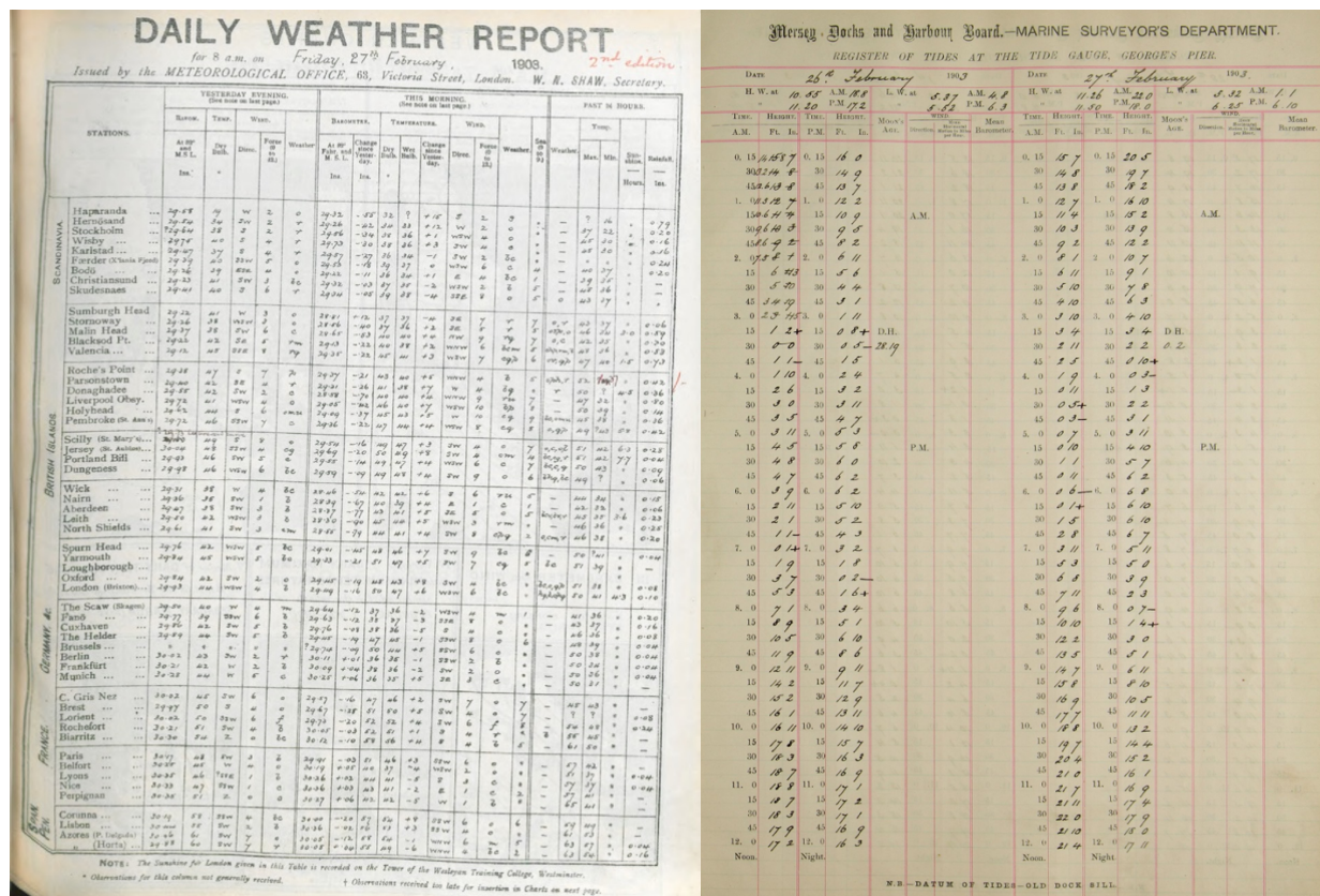
440 Figure A1: The UK Daily Weather Report observations page for 27 th February 1903 (left; from NMLA (2023)) and tide gauge measurements from Liverpool Docks for 26 th -27 th February 1903 (right; supplied by authors).
