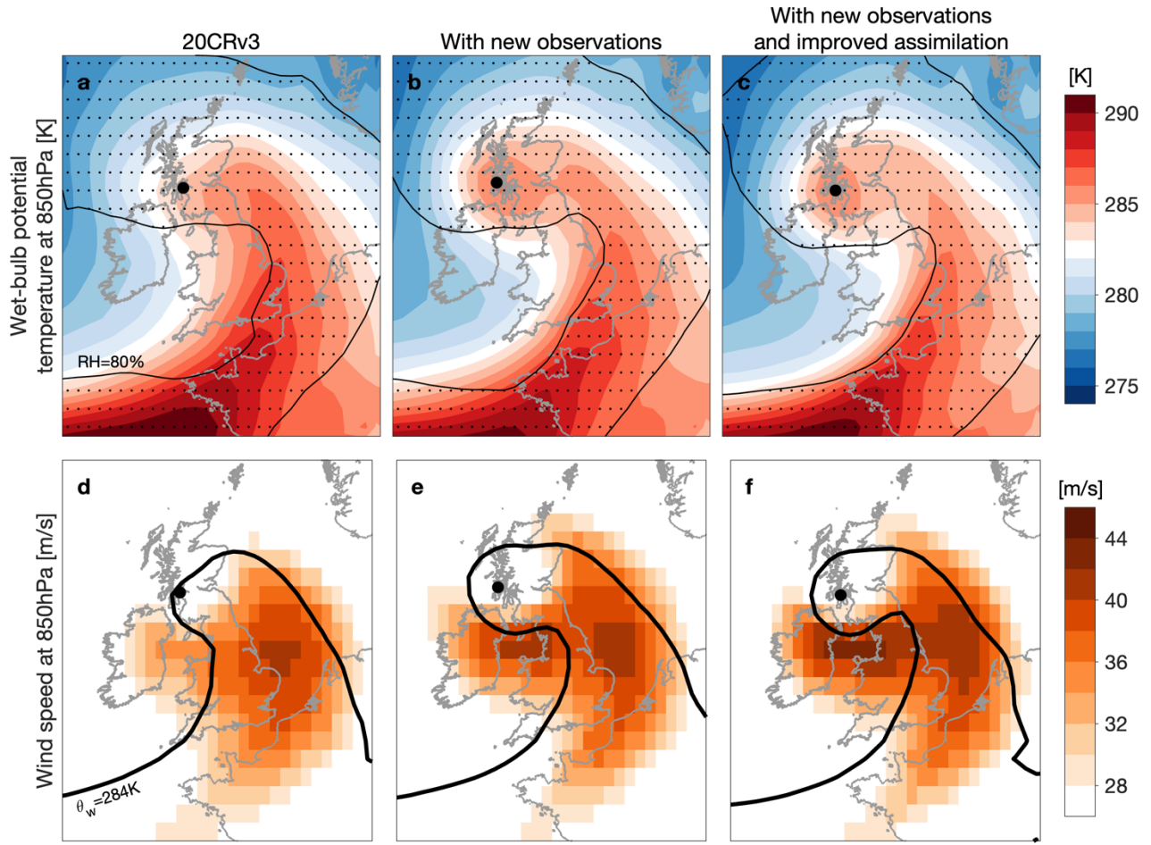
Figure 5: Ensemble mean of wet-bulb potential temperature at 850hPa (top row; a-c) and wind speed at 850hPa (bottom row; d-f) in the original 20CRv3 and two experiments with the reanalysis system (columns) at 0600 UTC on 27 th February 1903. The black filled circle represents the position of the mean sea level pressure minimum. The top panels also include stippling and a contour representing the location of the cloud head using relative humidity (RH) with respect to ice of above 80% at 700hPa. The 284K isotherm is indicated with the thick black contour in the bottom panels.
