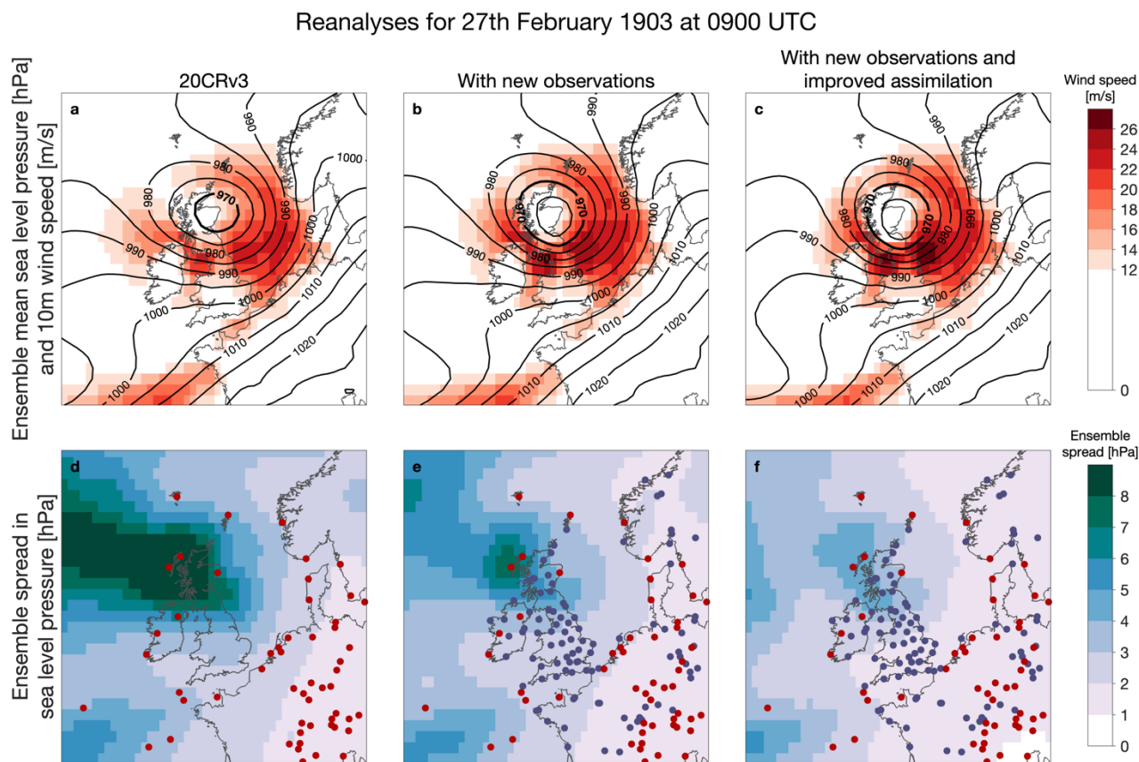
Figure 3: Reconstructing the atmospheric circulation during Storm Ulysses. Synoptic situation at 0900 UTC on 27 th February 1903. Isobars of sea level pressure (hPa; black contours) and wind strength at 10m (m/s; red shading) from the ensemble mean of 80 reanalysis fields are shown from 20CRv3 and the two different experiments (top row; a-c). Standard deviation of the ensemble of sea level pressure reanalysis fields ('ensemble spread') for the same time (hPa; blue shading; bottom row; d-f). Locations with available surface pressure observations in 20CRv3 are shown as red dots and new added observations in the experiments are shown as dark blue dots. Observations from both land stations and ships are shown, but there are very few available ship observations in this region at this time.
