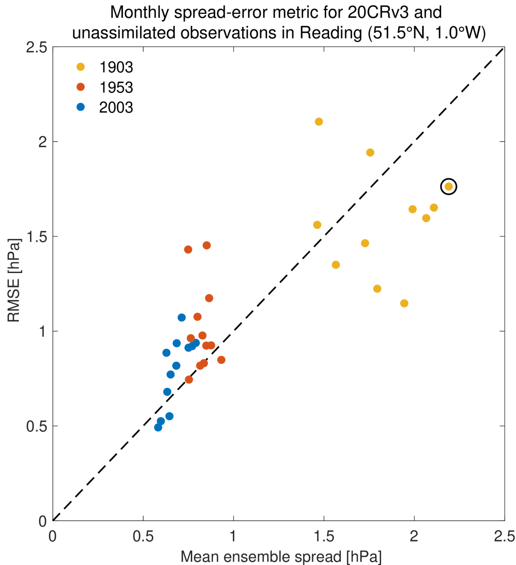
Figure B2: Ensemble reliability across years. Mean ensemble spread of the reanalysis, and RMSE of the reanalysis (both in hPa) compared to unassimilated independent observations from one location where data is available for an extended period (one dot per month from three different years). For the modern period (using 1953 and 2003 examples), the ensemble is roughly reliable so there is no evidence that the RTPS parameter needs to be altered for that time period. The open circle indicates February 1903.
