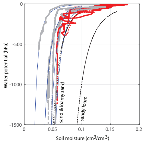
Figure 3. Estimates for the water retention curve of the applied soil. The red data has been obtained during the main experiment of this publication; at 30 cm depth a water potential Teros 21 sensor was installed about 15 cm apart from the soil moisture sensor. This is a rough estimate, as the sensors are not (and cannot be) installed directly next to each other. The gray curves were derived in other experiments with the same sand-potting soil ratio. All blue lines are fits that fall within the theoretical variations for sand and loamy sand, i.e. within the standard deviations of these soil types according to Clapp and Hornberger (1978)). The black curves are the curves for the average sand, loamy sand and sandy loam. Note that the graphs of other soil types such as clay/clay-sand are very different and not visible on these axes.
