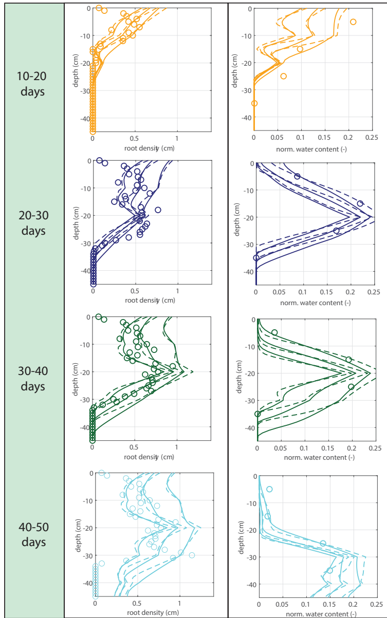
Figure 14. Comparison of results for loamy sand (solid lines) and sandy loam (dashed lines) for three different values for u_2 ( 0.6 \cdot 10^{-2} \text{ ml/cm/hr} , 1.2 \cdot 10^{-2} \text{ ml/cm/hr} and 2.4 \cdot 10^{-2} \text{ ml/cm/hr} ).
