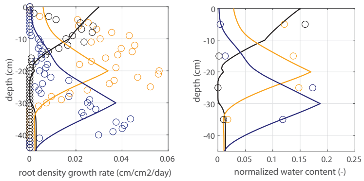
Figure 13. Model validation; results for the second data set using identical model parameters.
