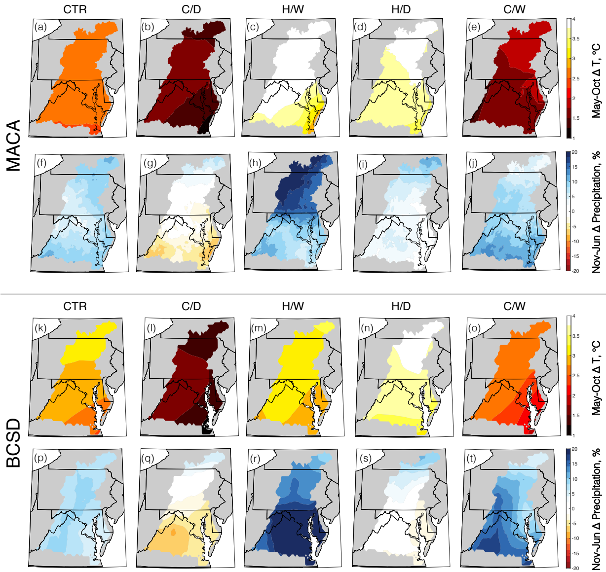
Figure S2: Relative changes in May to October temperatures (a-e, k-o) and November to June precipitation (f-j, p-t) for MACA (a-j) and BCSD (k-t) ESMs.
