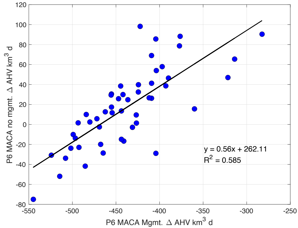
Figure S4: Relationship between MACA Phase 6 climate scenario \Delta AHV with and without the effects of management actions.
