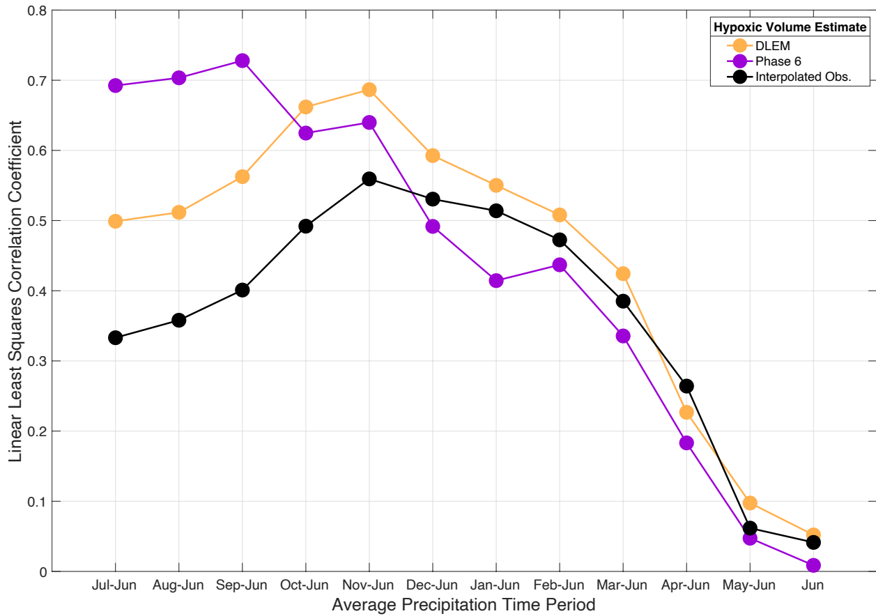
Figure S1: Correlation coefficients of annual hypoxic volume estimates (DLEM, Phase 6 and interpolated observations) as a function of average historical precipitation estimates for 1985-2014. The duration of average precipitation estimates decreases moving left to right, encompassing an entire year in the leftmost set of points and only accounting for June precipitation as a predictor of hypoxic volume in the rightmost set of points. The period November-June was chosen as the time period most predictive of AHV as it represents the highest correlations for both interpolated observations and DLEM hypoxia estimates, and has a comparable correlation for Phase 6 hypoxia.
