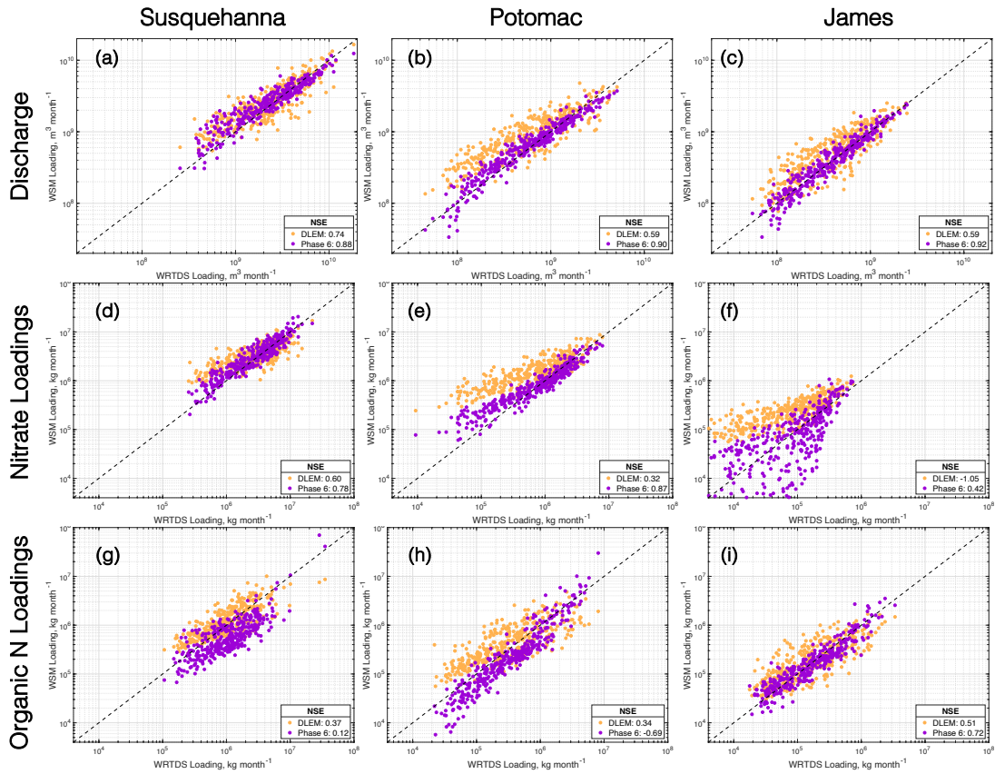
Figure S3: Comparison of monthly watershed model estimates vs. WRTDS derived observations for discharge (a-c), nitrate loadings (d-f) and organic nitrogen loadings (g-i) for the Susquehanna (a,d,g), Potomac (b,e,h), and James (c,f,i) tributaries at the respective river fall lines over the reference period 1991-2000. Nash–Sutcliffe Efficiencies (NSE) reported in bottom right of each panel for both watershed models.
