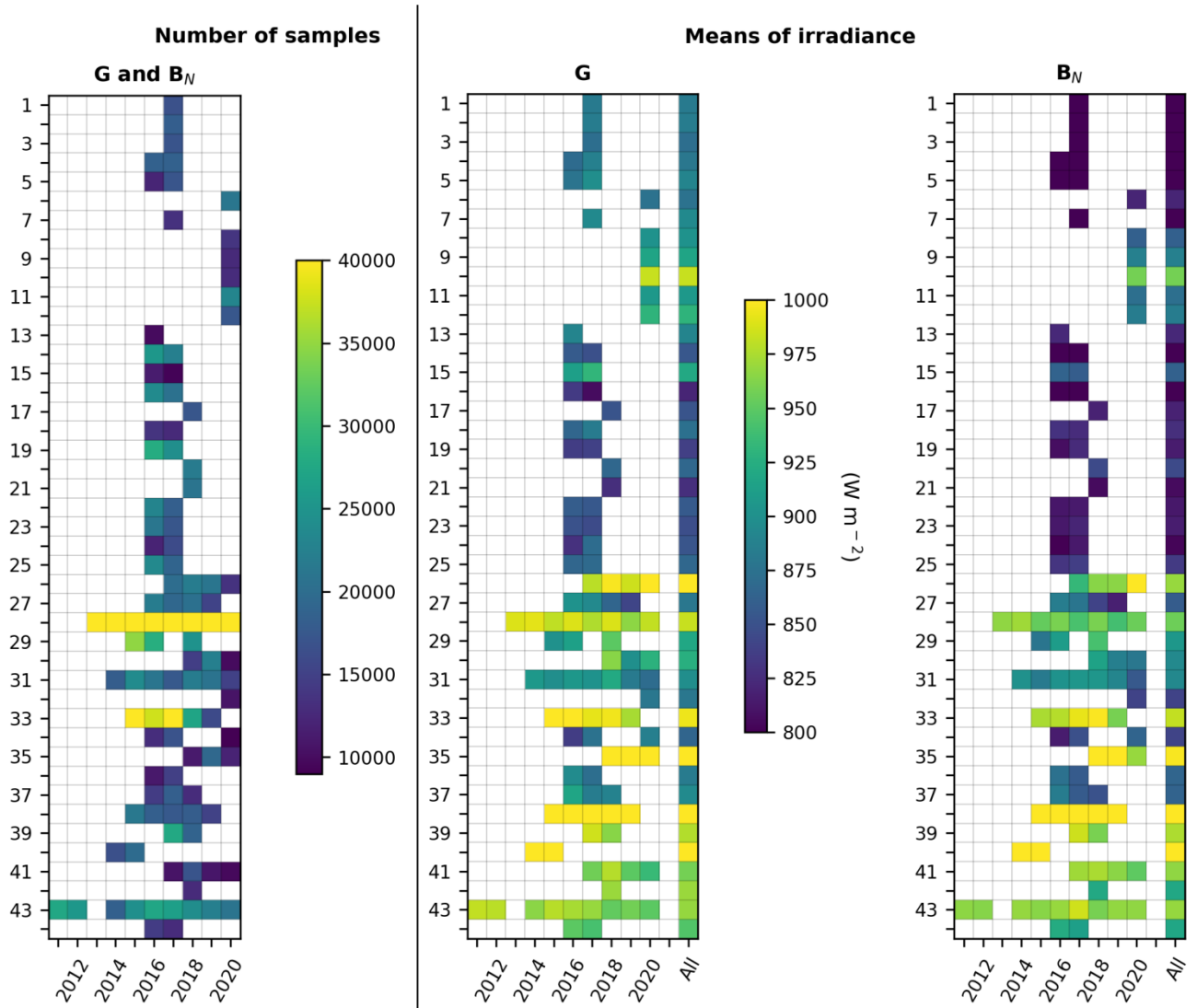
355 Figure 2: Number of retained measurements (left) and means of G and B_N (right) at each station for each year. Also reported are the means for G and B_N for the whole period (All). Numbers refer to the rank of the station in Table 1.
