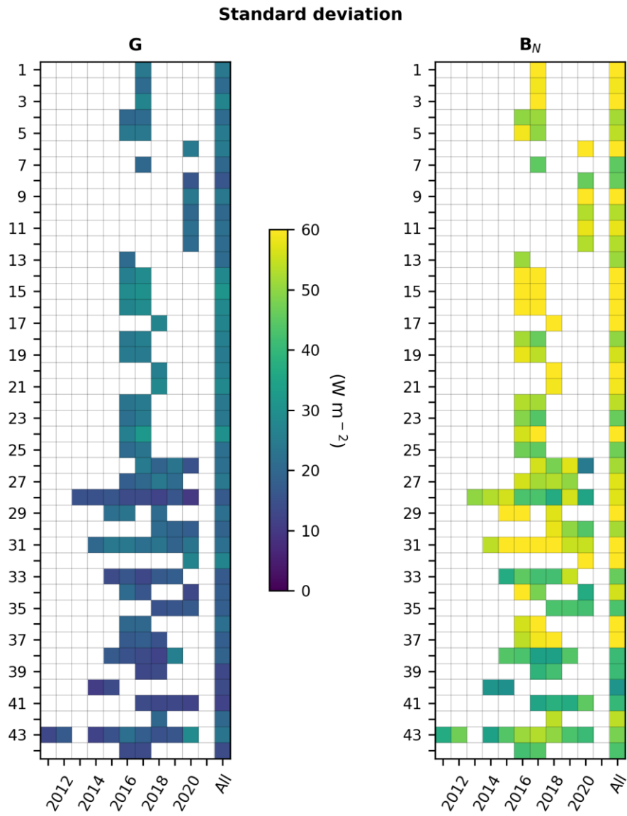
615 Figure 7: Standard deviation of errors for G and B_N at each station for each year, and for the whole period (All). Numbers refer to the rank of the station in Table 1.
