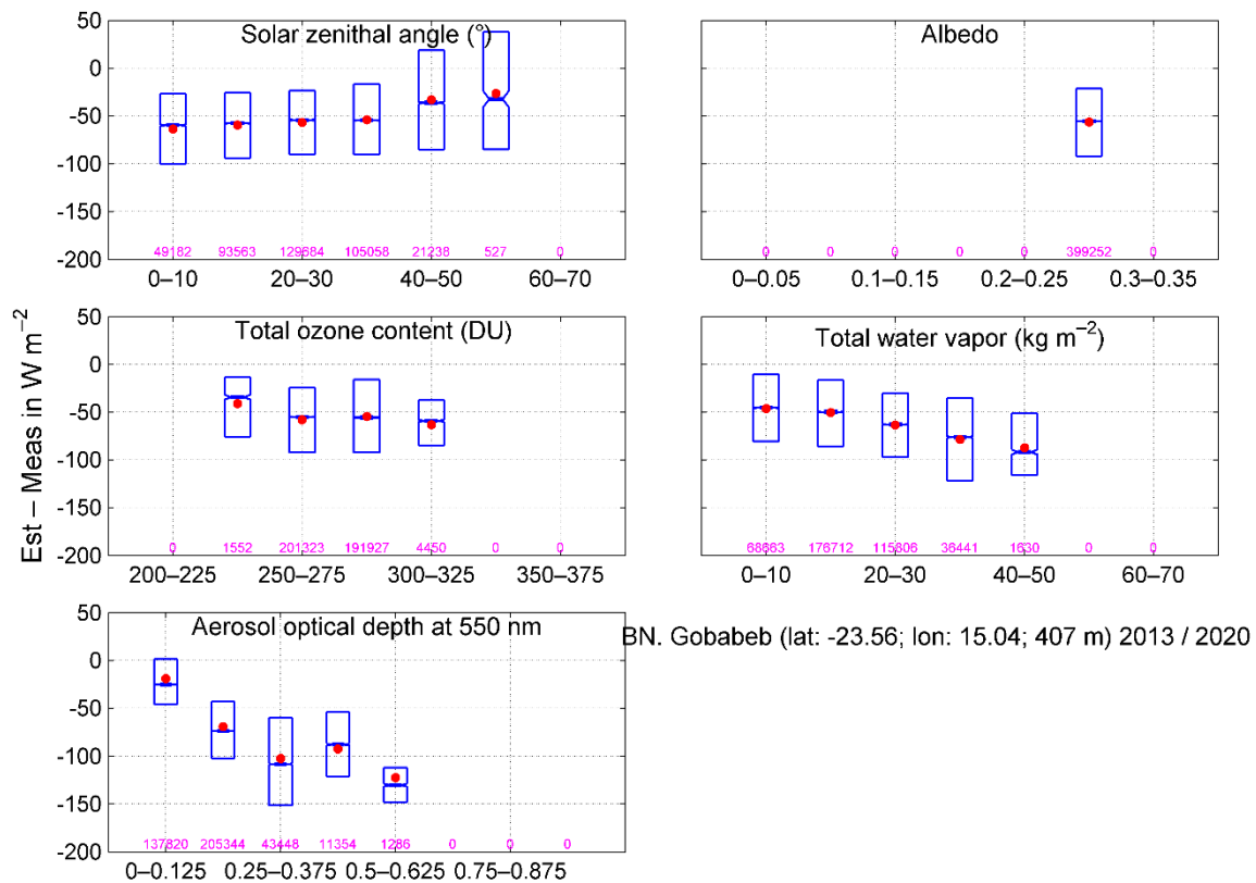
795 Figure 5-10: Boxplots of the differences between the McClear estimates and the measurements of B_N at the BSRN station Gobabeb (#28, climate BWh) for several classes of various variables. In each boxplot, the red point is the mean while the lower, middle and upper lines are respectively the 25, 50 and 75 percentiles. The number of samples is given for each class. Only classes with at least 50 samples are drawn.
