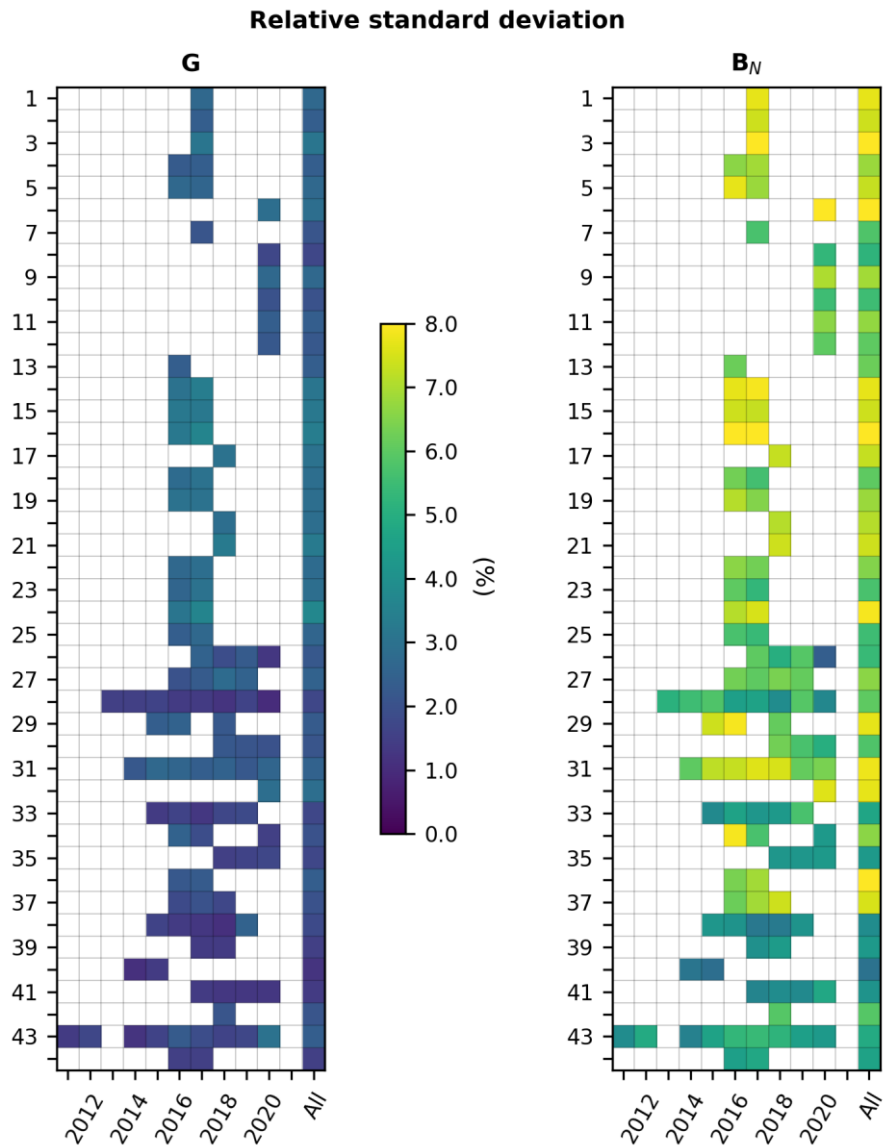
1125 Figure A58: Relative standard deviation of errors for G and B_N at each station for each year, and for the whole period (All). Numbers refer to the rank of the station in Table 1.
