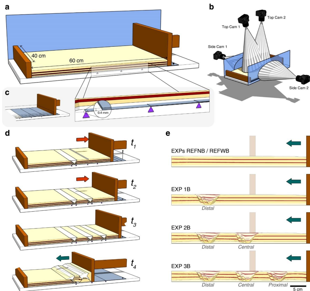
815 Figure 2. Modelling set-up. (a) Sketch of the employed apparatus, oblique view. (b) Sketch showing the overall camera setup for PIV processing. (c) Close up view of the basal sheets system. Triangles indicate the end of each sheet. (d) Illustrated example showing the steps involved in the basin formation -extension- and basin inversion -shortening- stages of the experiments. (e) Summary of initial conditions for the shortening experiments.
