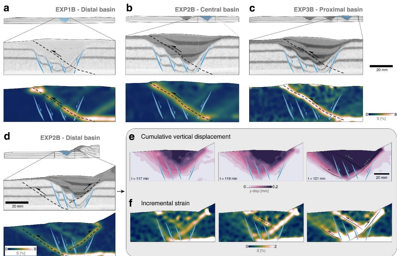
885 Figure 10. Close up view to selected basins, highlighting thrust localisation. (a) Experiment 1B, distal basin. (b) Experiment 2B, central basin. (c) Experiment 3B, proximal basin. (d) Experiment 2B, distal basin. (e) Close-up view visualizing different time increments for cumulative vertical displacement and (f) incremental strain of the distal basin in EXP2B.
