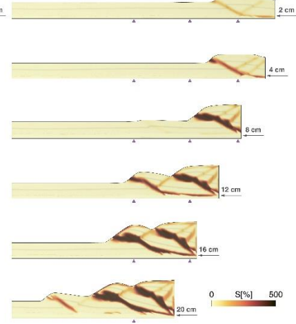
855 Figure 4. Deformation evolution, comparison between reference experiments. Experiment REFNB, no basal sheet; (a) side-view photographs, (b) incremental strain, and (c) cumulative strain. Experiment REFNB, with basal sheet; (d) side-view photographs, (e) incremental strain, and (f) cumulative strain.
