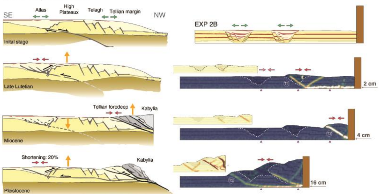
895 Figure 12. Temporal evolution comparison between selected natural examples and our analogue modelling results. (a) Carpathians vs EXP3B (redrawn from Picha et al., 2006). MF: Magura Flysch, SU: Silesian Unit. (b) Atlas vs EXP2B (redrawn from Bracene & de Lamotte, 2002)
