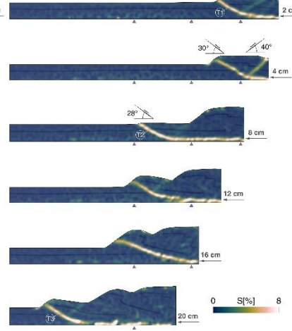
855 Figure 4. Deformation evolution, comparison between reference experiments. Experiment REFNB, no basal sheet; (a) side-view photographs, (b) incremental strain, and (c) cumulative strain. Experiment REFNB, with basal sheet; (d) side-view photographs, (e) incremental strain, and (f) cumulative strain.
