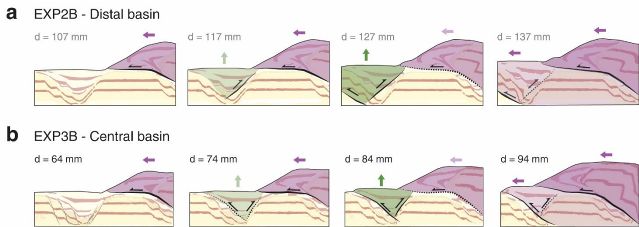
890 Figure 11. Interpreted sections of selected experiments showing thrust sheet progression and impact on basin inversion. (a) Experiment 2B, distal basin. (b) Experiment 3B, central basin.
