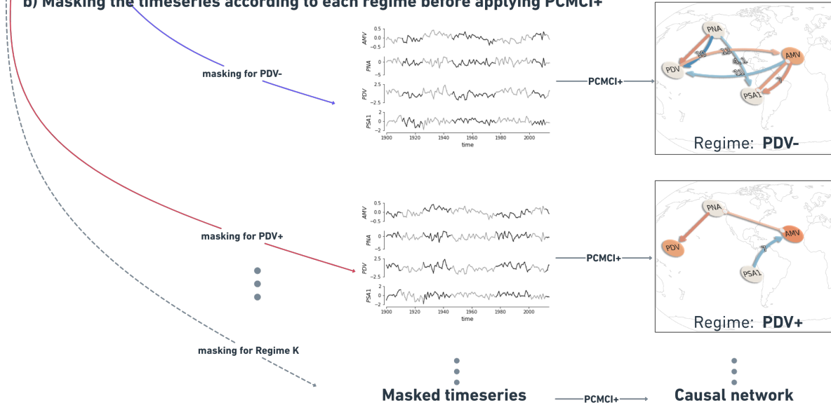
Figure 3. a) PDV and AMV timeseries calculated by CVDP-LE diagnostics on ERSSTv5 data are smoothed using 11 and 13-year low-pass filters, respectively. 10 regimes are defined (see table on the left) in addition to the 1900-2014 complete period. The PCMCi+ algorithm is applied on unfiltered (non-smoothed) PDV, AMV, PNA, PSA1 yearly detrended timeseries that are masked according to the periods that define each regime. The right arrows on the smoothed timeseries represent unmasked periods from three out of 10 regimes (PDV+/AMV+, PDV-/AMV+, and PDV+/AMV-). b) The regimes identified in (a) are used to mask the non-smoothed (but detrended) index timeseries before applying PCMCi+. Here, for example, we show how we mask the data according to the PDV- (top) and PDV+ (bottom) regimes. The grey shaded periods are masked and thus not considered during the PCMCi+ analysis. Note that the masking here refers to variables at time point X_t^j while their lagged parents can originate also from a masked period (gray shaded). This setting is referred to as mask_type='y' in Tigramite. Consequently, applying PCMCi+ on differently-masked timeseries produces different causal networks (network in top vs network in bottom)
