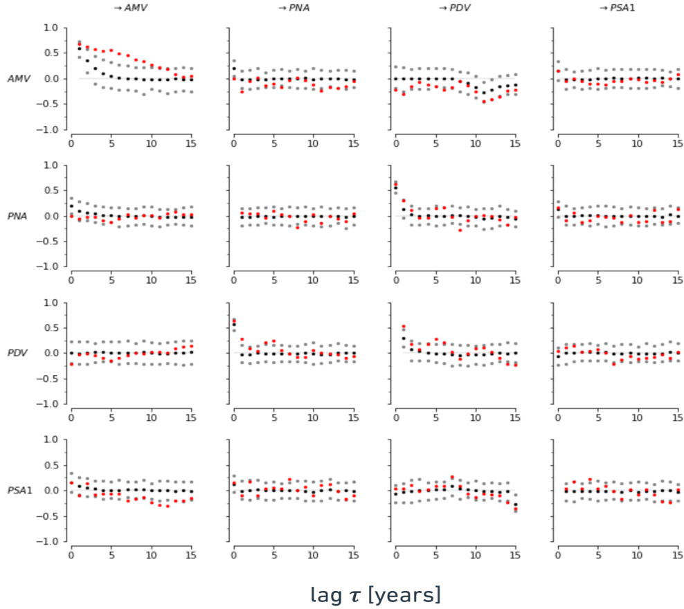
Figure 6. Lagged correlations of original data (complete period graph from reanalysis data) in red shown together with lagged correlations of an ensemble of synthetic data generated by a linear Gaussian structural causal model with causal coefficients and noise structure estimated from the original data. The mean lagged correlations from the synthetically generated data are shown in black, and their 5th-95th percentile range in grey. Lagged correlations of original data (lag in years, complete period graph from reanalysis data) in red shown together with lagged correlations of an ensemble of synthetic data generated by a linear Gaussian structural causal model with causal coefficients and noise structure estimated from the original data. The mean lagged correlations from the synthetically generated data are shown in black, and their 5th-95th percentile range in grey. X-axis shows lag in years.
