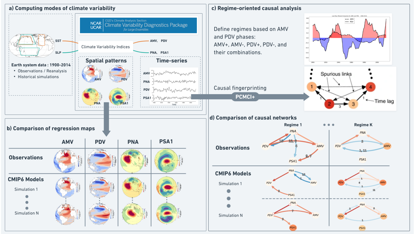
Figure 1. Framework for the regime-oriented causal model evaluation. a) Gridded SST and SLP data used to calculate indices for AMV, PDV, PNA and PSA1 modes of climate variability. Diagnostics from the NCAR Climate Variability Diagnostic Package for Large-Ensembles (CVDP-LE) produce the timeseries of these indices and their associated spatial patterns (regression maps). b) We first, as a sanity check, compare the CMIP6 model-simulated SST (for AMV and PDV) and SLP (for PNA, PSA1) regression maps to those from reanalysis before c) using the timeseries of the four indices for the regime-oriented causal analysis. Here we define different regimes depending on the sign of the 13-year low-pass filtered AMV and 11-year low-pass filtered PDV timeseries. For every regime we run PCMCi+ to estimate instantaneous and lagged links between nodes representing the timeseries of the indices calculated in (a) from the reanalyses and model data. In this schematic example, there are four indices, with node color indicating auto-correlation, and there is a causal link (solid black arrow) between index 2 and indices 1 and 3, and then there is a causal link between indices 3 and 4. The method identifies and removes spurious links (see black dashed arrows) between indices 1 and 4, or 2 and 4. Unitless representative time lags are labeled on each causal link, where index 1 lags index 2 by one time-step (depending on temporal resolution of the timeseries, here yearly), index 3 lags index 2 by three, and index 4 lags index 3 by one. Applying the method to the timeseries in (a) provides d) dataset- and regime-specific causal fingerprints in a similar format to the schematic in (c), which can be used for model evaluation and intercomparison. We calculate annual averages from the monthly timeseries of PDV and AMV provided by CVDP-LE. This way, the dataframe is fit for multi-year and decadal causal estimations. In addition to the subtraction of global mean temperatures in the CVDP-LE calculation of PDV and AMV, the causal networks are estimated after linearly detrending the timeseries of the four indices to ensure their stationarity. The estimated causal dependencies (links) are hence assumed to be a mixture of internal variability and time-varying anthropogenic forcing (mainly from aerosols).
