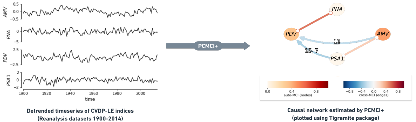
Figure 2. Constructing causal network using Tigramite by applying PCMCi+ on timeseries calculated by CVDP-LE from reanalysis datasets. Each node on a causal network (right) represents a variable (timeseries, left) and the node color its auto-correlation (self links of each variable). The link color shows the cross-MCI partial correlation value which denotes the sign and strength of the estimated causal link between two variables. The time lag for lagged links (curved arrows) are shown as small labels on the links. Straight lines represent instantaneous causal links happening with no time lag.
