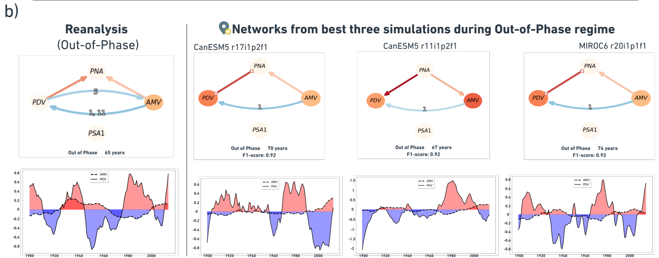
Figure 8. a) Whisker plot showing the distribution of F_1 -scores across the CMIP6 LEs for the causal analysis for: the complete period (light blue boxes), the In-Phase regime (dark blue boxes) and the Out-of-Phase regime (green boxes). White scatter points denote the mean LE F_1 -scores. b) Reference causal network estimated from reanalysis during the Out-of-Phase regime (left, with low-pass AMV and PDV timeseries below) compared to networks and timeseries from three CMIP6 simulations (right, with simulated low-pass AMV and PDV timeseries below each network) with the best network similarity i.e. highest F_1 -score.
