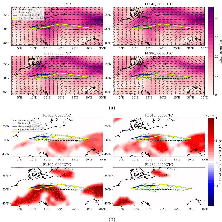
Figure 10. Lateral paths for Scenario I (13 th of June 2018, 0000UTC) depicted with (a) wind and (b) aCCF of contrails as colormaps.
