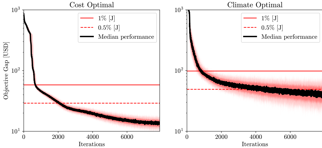
Figure 8. Sensitivity of the convergence performance of the optimization algorithm to 50 different executions for the cost and climate optimal routing options ( \alpha = 1 and \alpha = 0 , respectively)(1 iteration \approx 4 ms). The objective gap is calculated considering the deviations from the best performance obtained among 50 runs (i.e., the minimum value of J ) as the reference, i.e., at each iteration, the value of the objective function (used for trajectory optimization Eq. (17)) is compared with the minimum value obtained from other executions. The mean value is highlighted in a solid black line, and 0, 10, 90, and 100 percentiles are represented with different color bands.
