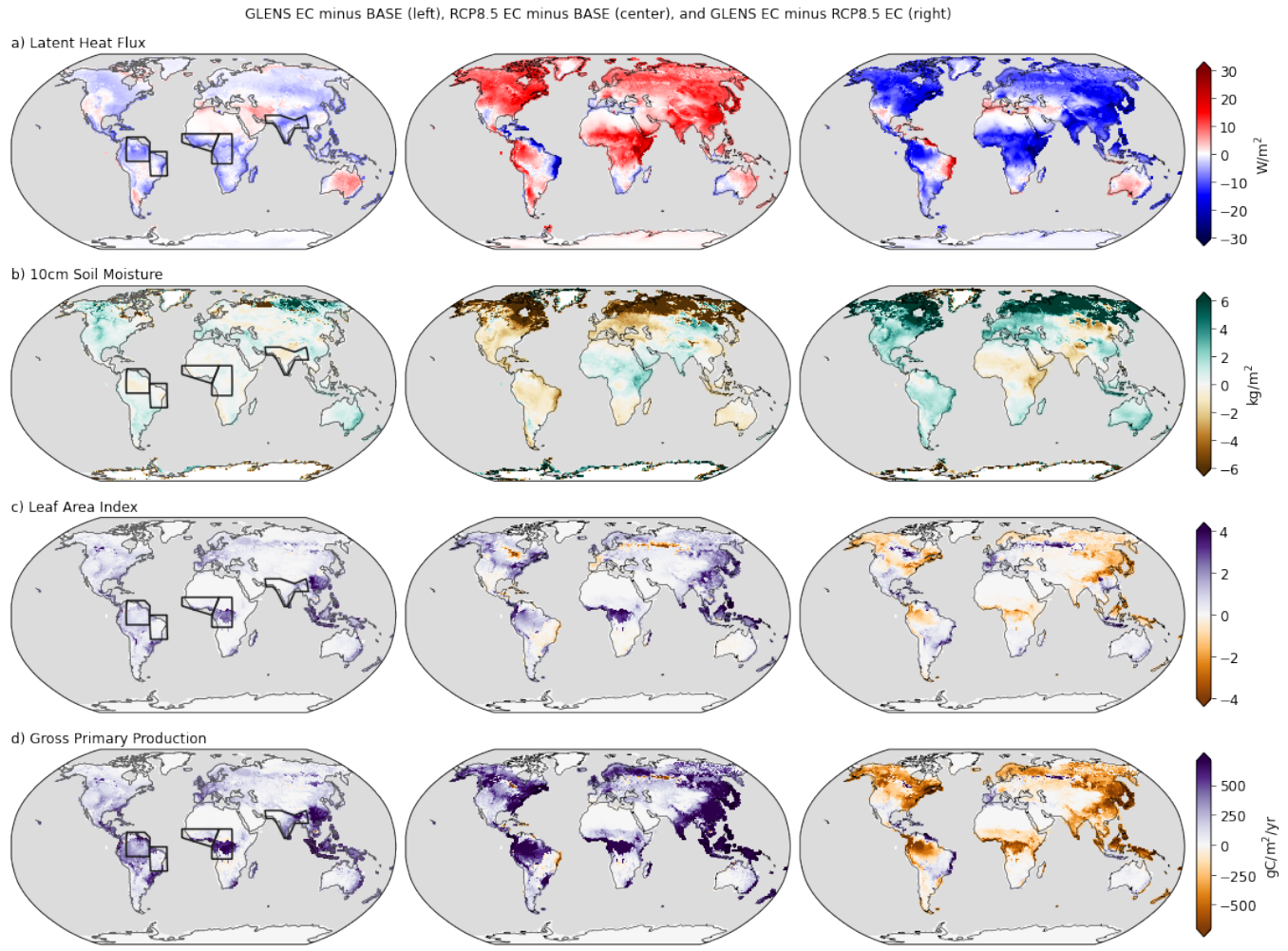
Figure 10: Projected changes between GLENS EC (2075-2095) and BASE (2010-2030) in the left column , changes between RCP8.5 EC (2075-2095) and BASE (2010-2030) in the center column , and changes between GLENS EC (2075-2095) and RCP8.5 EC (2075-2095) in the right column , for in a) latent heat flux; b) soil moisture in the top 10cm; c) total leaf area index; and d) gross primary production. Black polygons in the left column highlight the following regions: Northeast South America ( NESNSA ), North South America ( NSA ), Western Africa ( WAF ), Central Africa ( CAF ), and South Asia ( SAS ).
