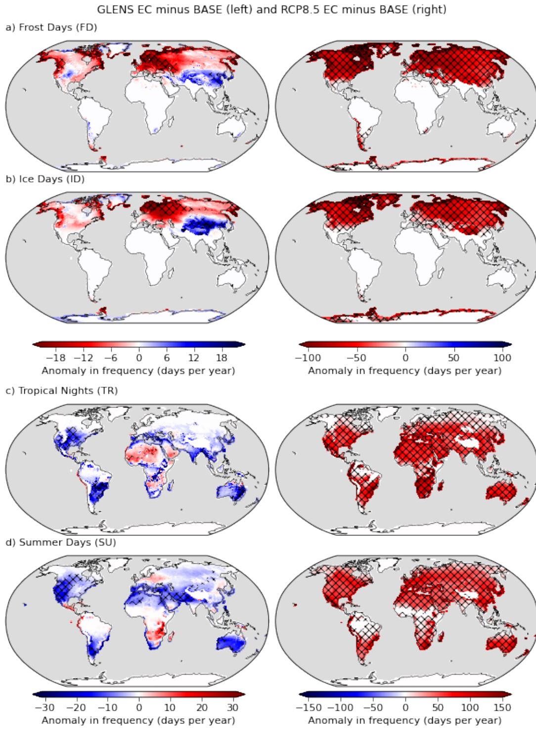
29 Figure 4: The same as Figure 2, but containing projected anomalies in the number of days per year with 30 frequency of daily minima <0^{\circ}\text{C} (frost days, FD), daily maxima <0^{\circ}\text{C} (ice days, ID), daily minima >20^{\circ}\text{C} 31 (tropical nights, TR) and daily maxima >25^{\circ}\text{C} (summer days, SU). Hatching indicates significance at the 5% 32 test level using the Student's t-test.
