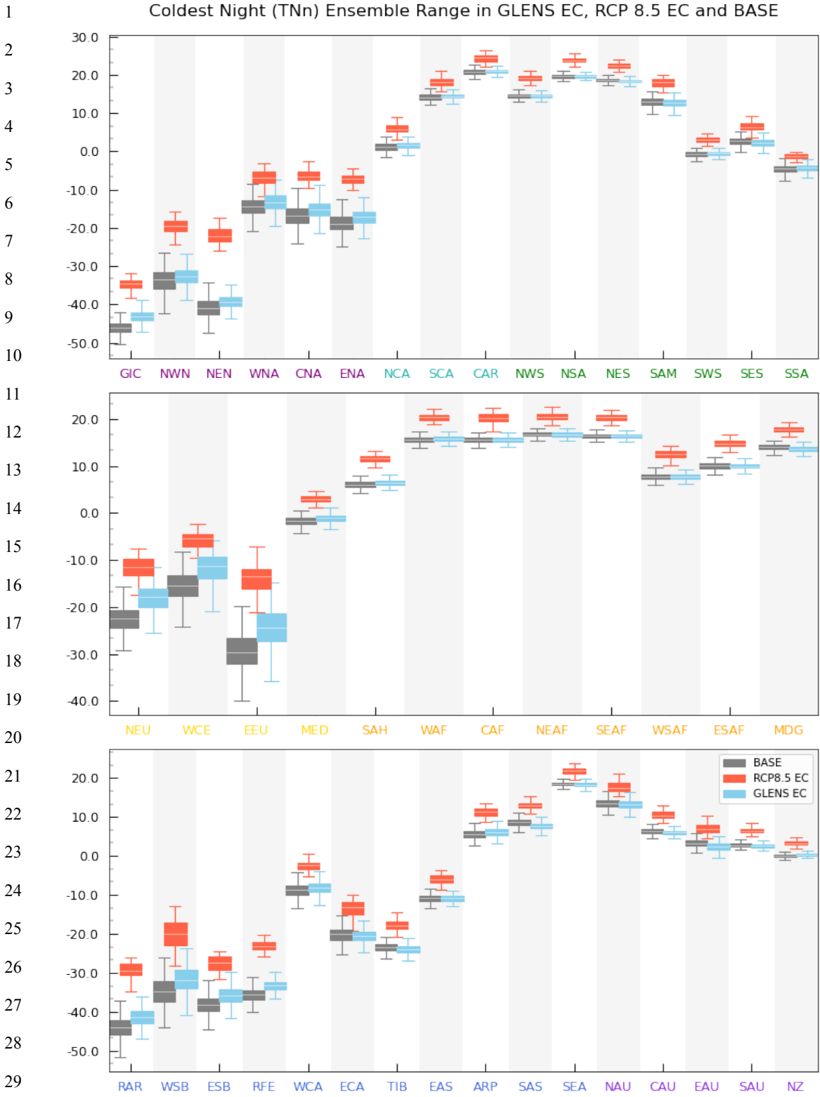
Figure 3: Climatological mean of coldest night (TNn) for: BASE (2010-2030) in grey, GLENS End of Century (EC; 2075-2095) in blue and RCP8.5 EC in red in each of the AR6 regions except Antarctica (Iturbide et al., 2019). Boxes show ensemble mean in white with the limits set at 25% and 75% of the ensemble spread; whiskers denote 5% and 95% ensemble spread.
