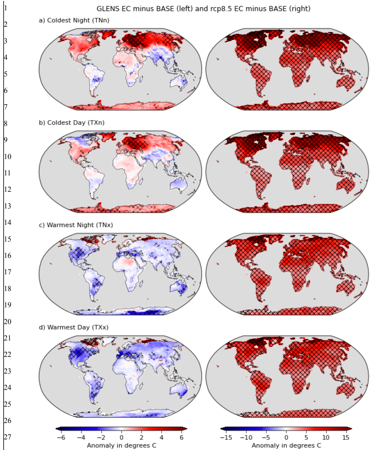
Figure 2: Projected anomalies between the GLENS EC scenario (2075-2095) and BASE (2010-2030) for annual coldest night and day (TNn, TXn), and warmest night and day (TNx, TXx) shown in the left column, and for anomalies between RCP8.5 EC (2075-2095) and BASE (2010-2030) shown in the right column. Note that the colorbar is different in the right column. Hatching indicates significance at the 5% test level using the Student's t -test.
